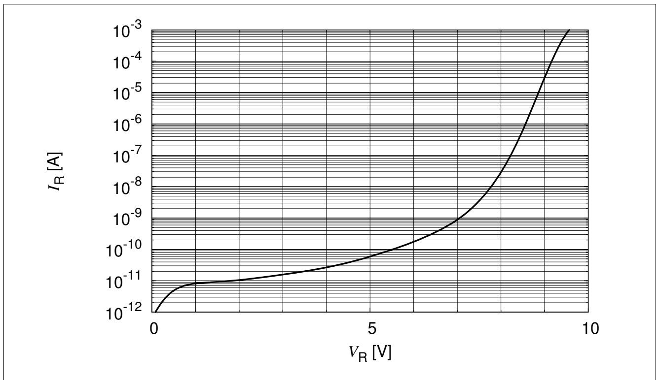
Figure 8 Reverse characteristic, I_R = f(V_R) , voltage forced
