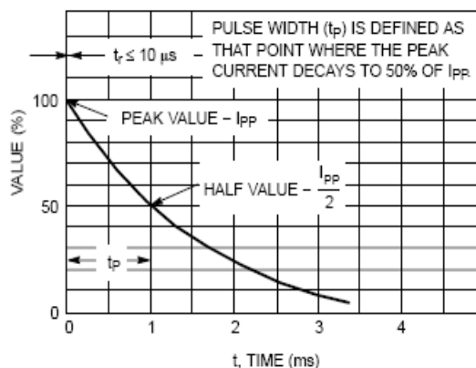
Figure 2. 10 x 1000 \mu s Pulse Waveform
