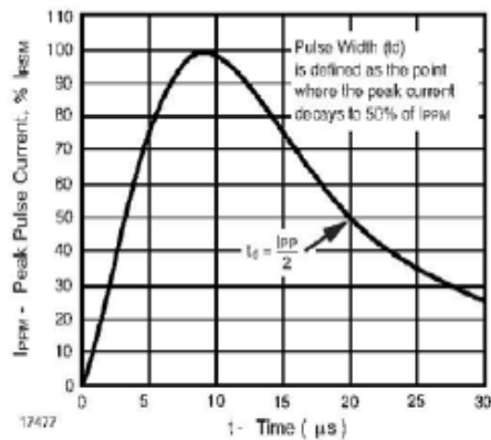
Figure 2. Pulse Waveform
