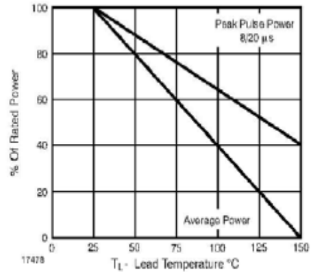
Figure 3. Power Derating
