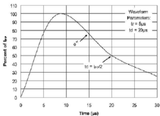
Pulse Waveform
