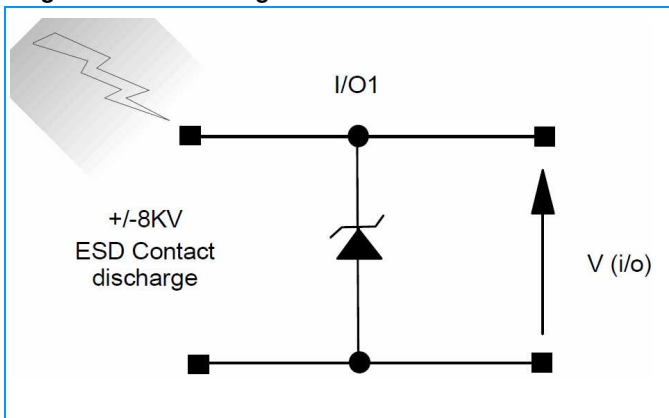
Fig7. ESD Test Configuration
