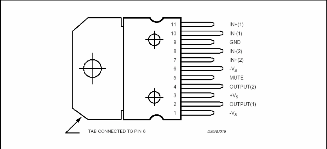
PIN CONNECTION (Top view)
