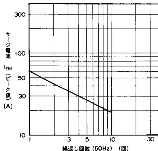
Surge Capability
