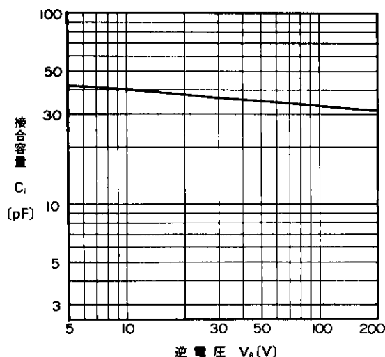
Junction Capacitance
