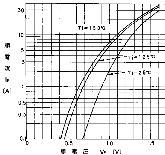
Forward Characteristics
