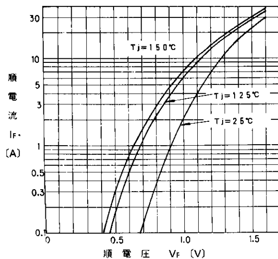
Forward Characteristics
