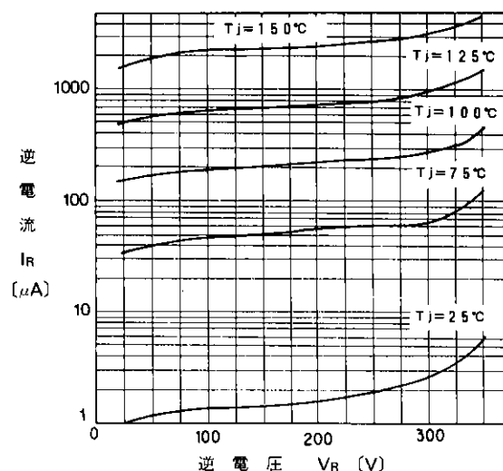
Reverse Characteristics
