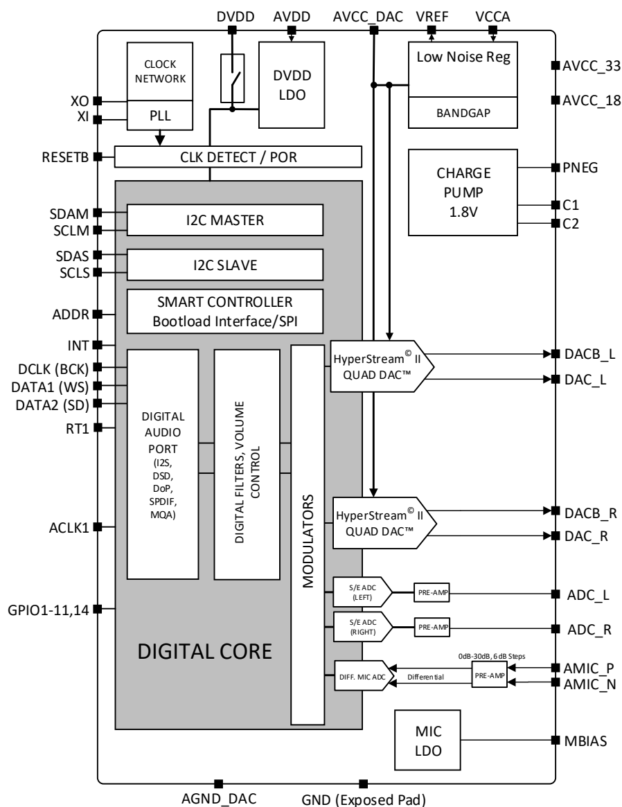
Figure 1 - ES9068A Block Diagram
