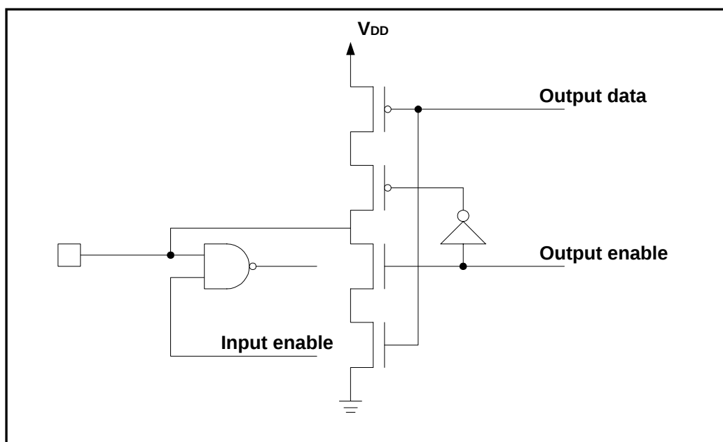
Input/Output Pin Configuration
