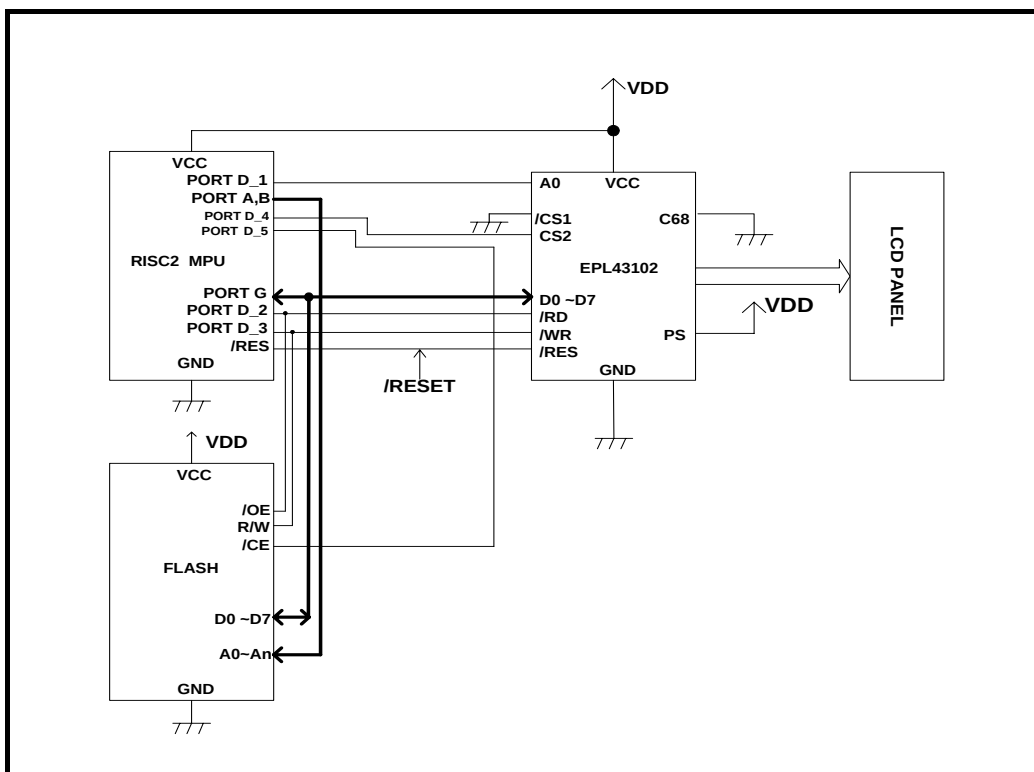
Elan 8-bit MPU ( with external memory )
