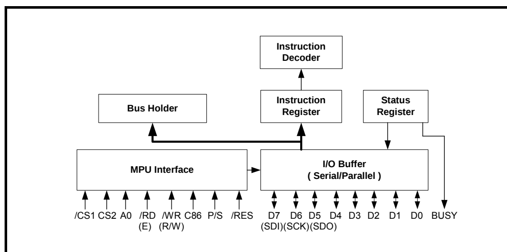
Figure 7-1 System Interface
