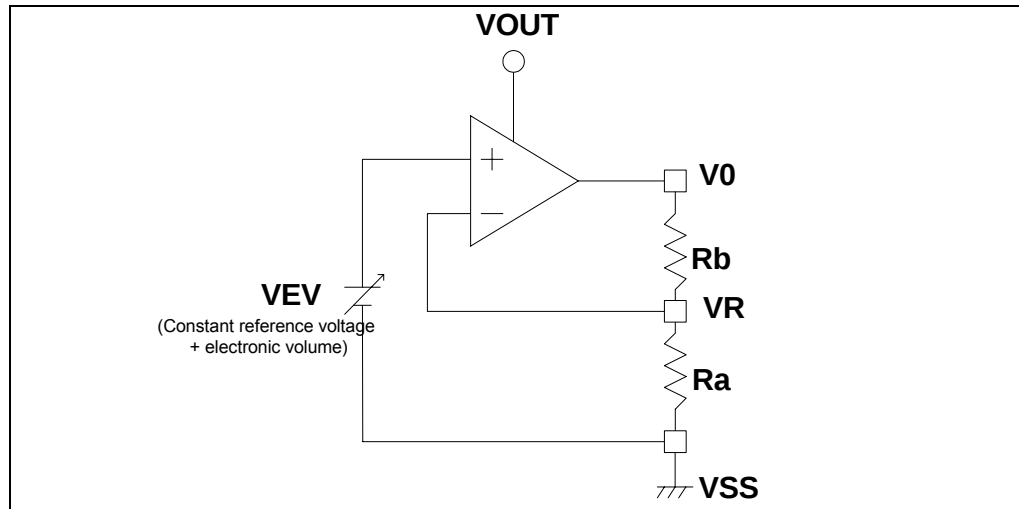
Figure 7-15 Resistor Connection
