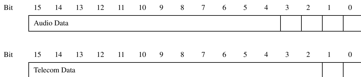
Figure 3-6. Format for the Audio and Telecom FIFOs
