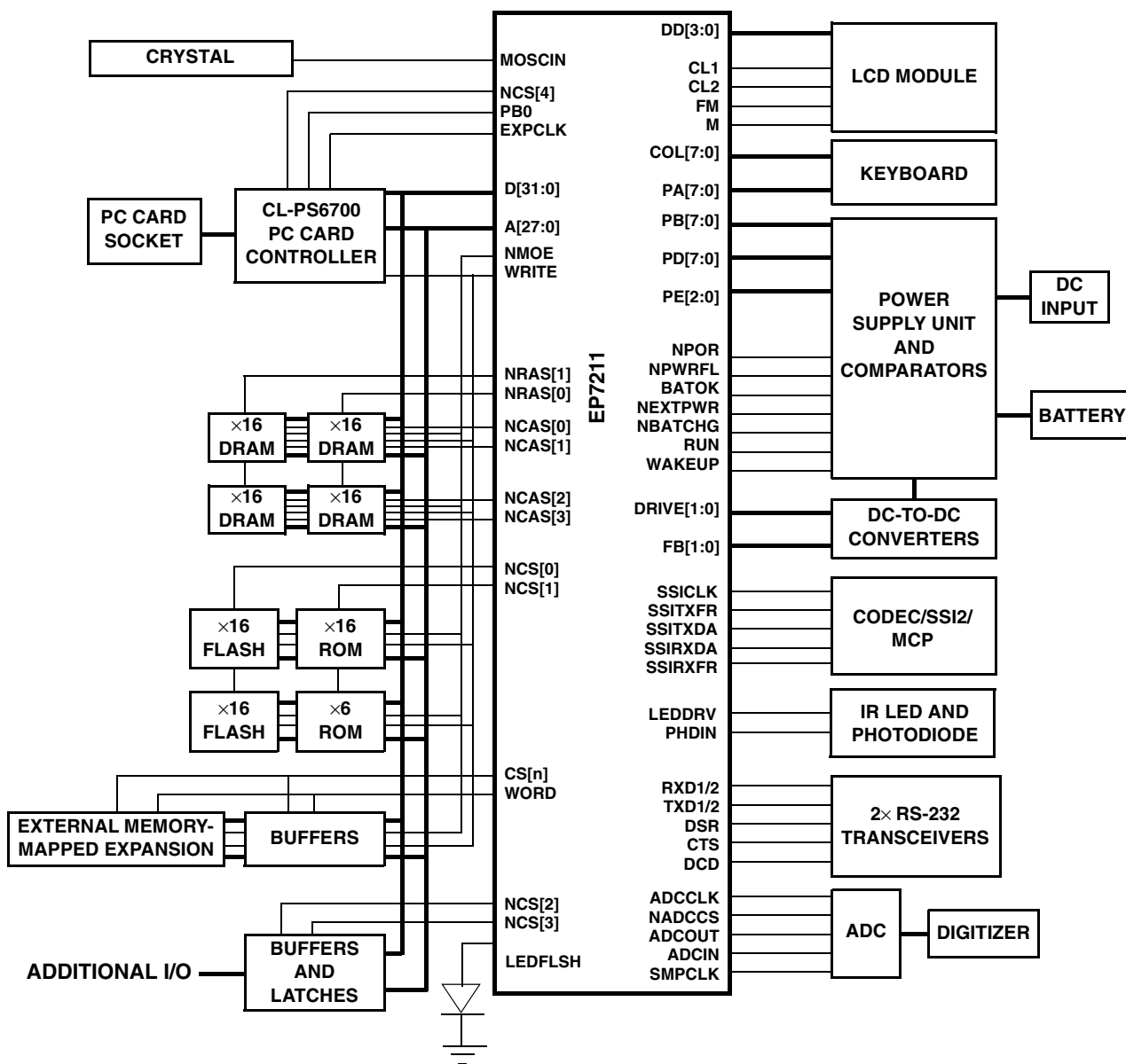
Figure 3-13. A Maximum EP7211 Based System
