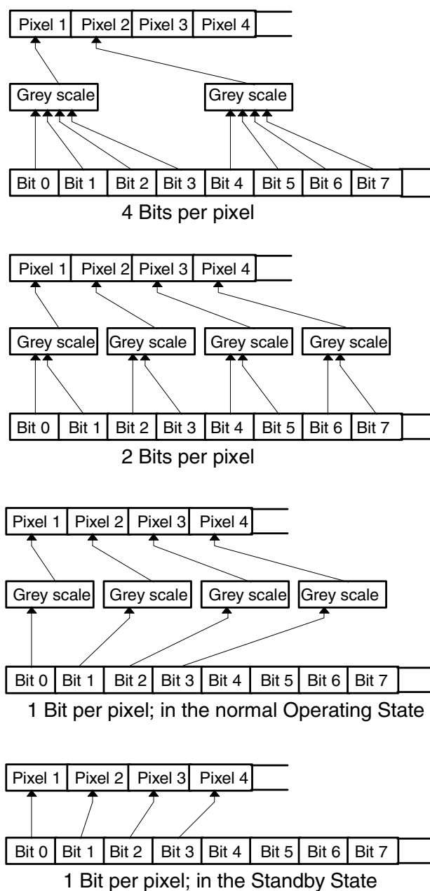
Figure 3-9. Video Buffer Mapping shows the organization of the video map for all combinations of bits per pixel.
