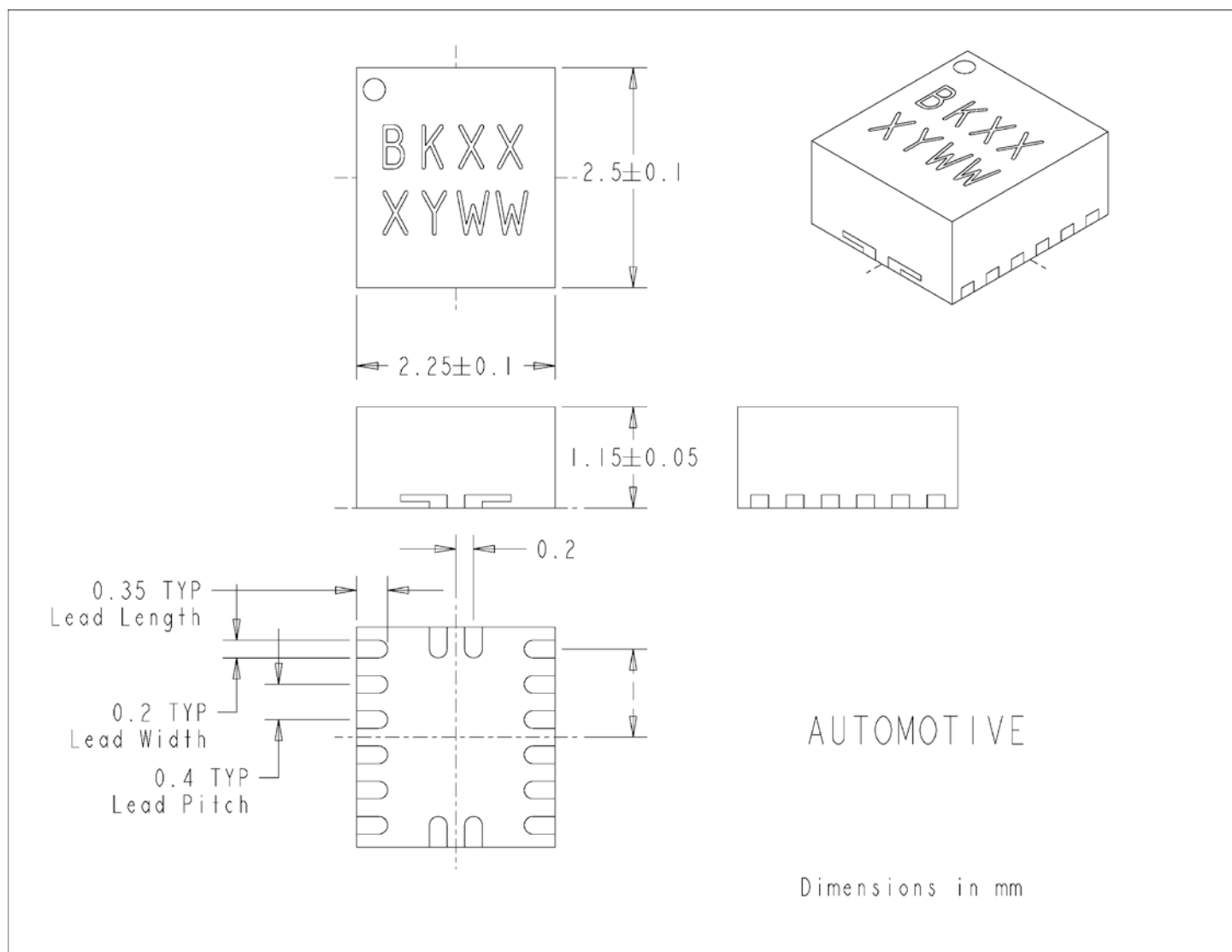
Figure 13. EP5358LUA Package Dimensions (Bottom View)
