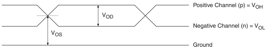
Figure 11–6. Transmitter Output Signal Level Waveforms for RSDS
