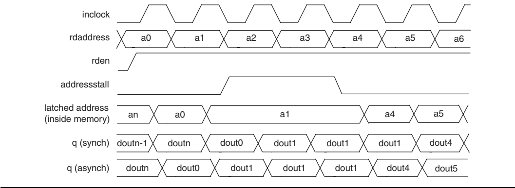
Figure 8–4. Cyclone II Address Clock Enable During Read Cycle Waveform
