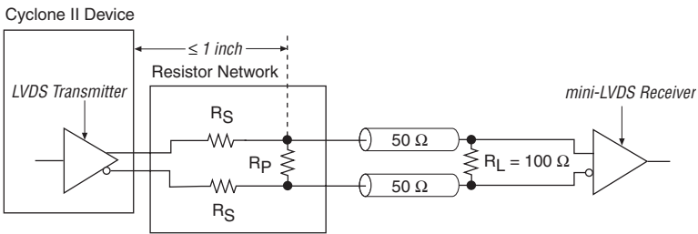
Figure 11–10. mini-LVDS Resistor Network
