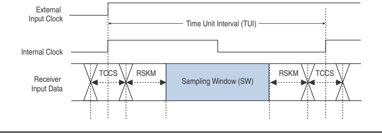
Figure 5–3. High-Speed I/O Timing Diagram
