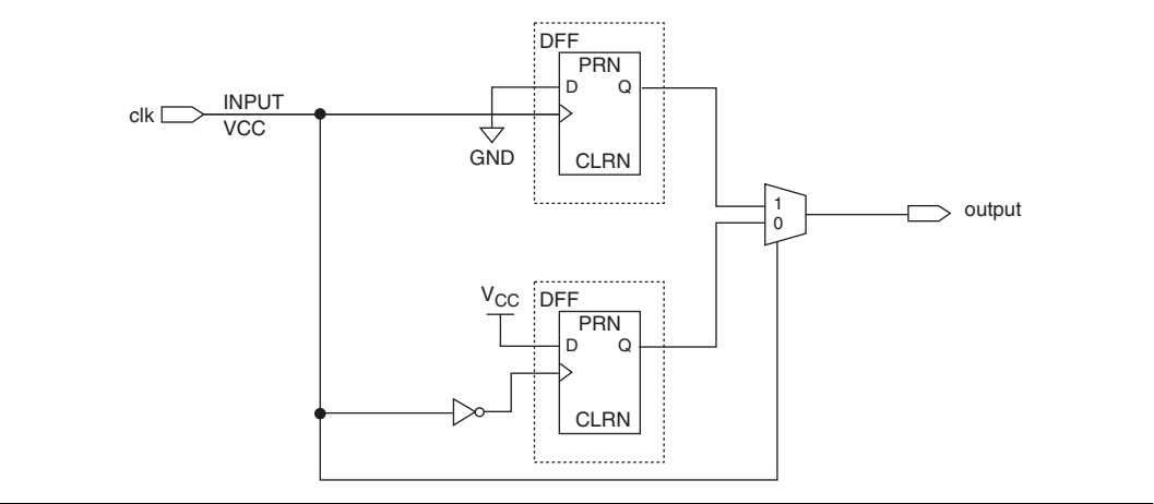
Figure 5–10. DCD Measurement Technique for DDIO (Double-Data Rate) Outputs
