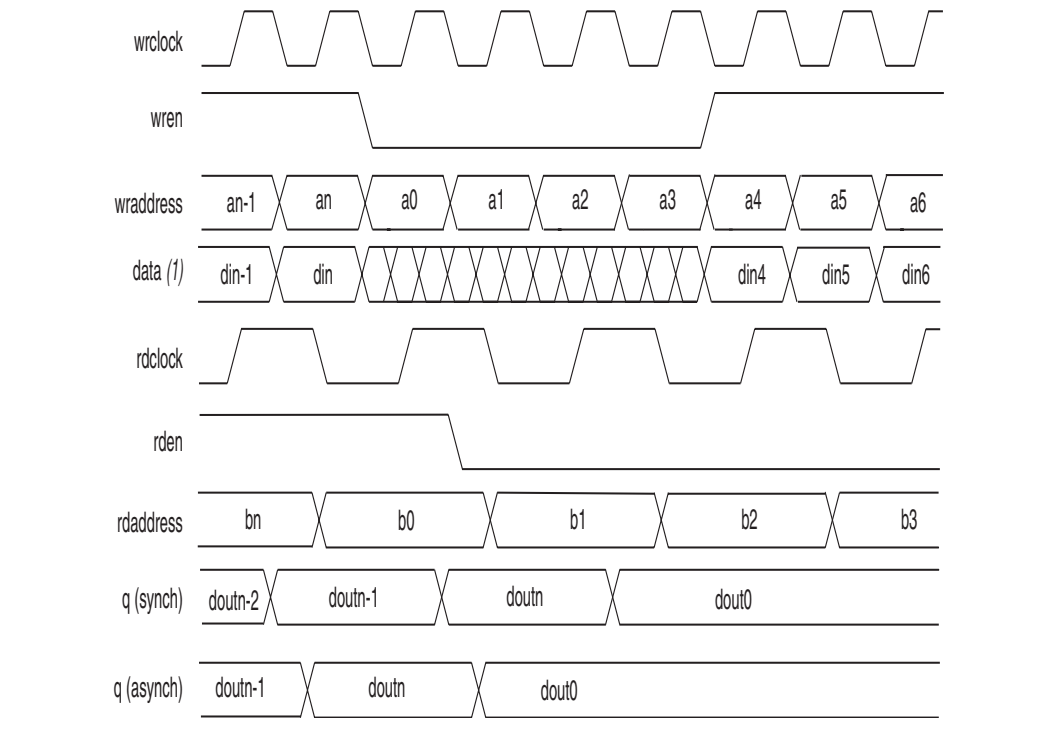
Figure 8–12. Cyclone II Shift Register Mode Configuration
