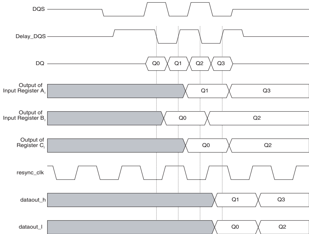
Figure 9–12. DDR Input Functional Waveforms
