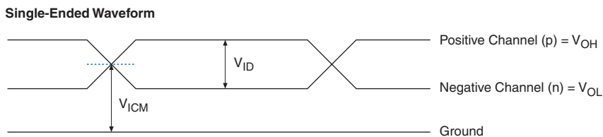
Figure 11–4. Receiver Input Waveforms for the LVDS Differential I/O Standard
