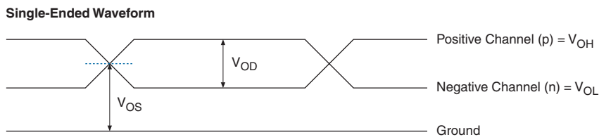
Figure 11–5. Transmitter Output Waveform for the LVDS Differential I/O Standard Note (2)
