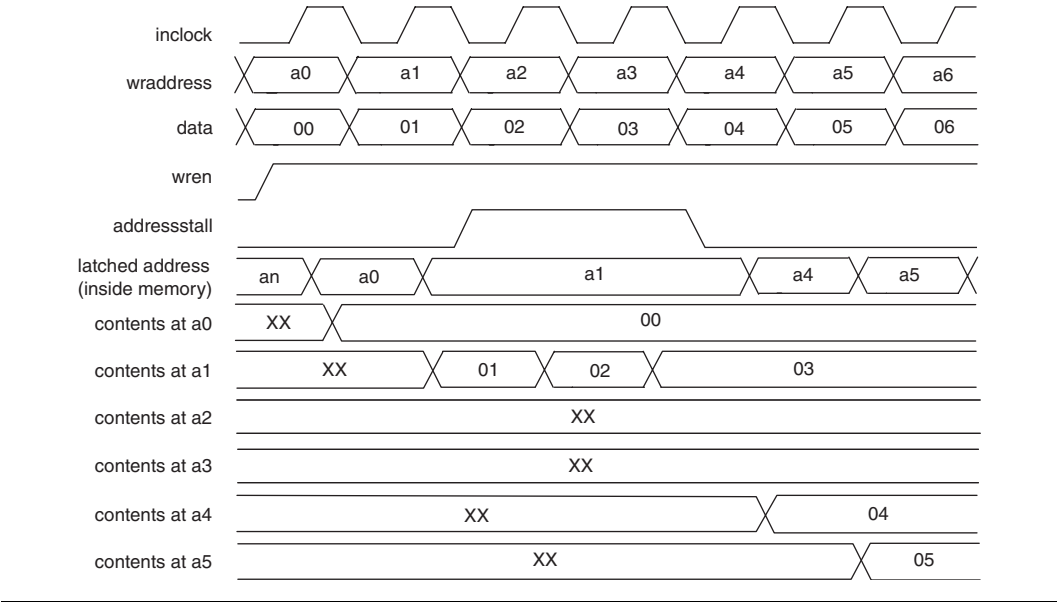
Figure 8–5. Cyclone II Address Clock Enable During Write Cycle Waveform
