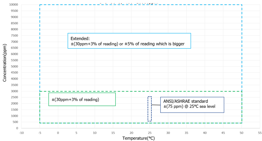
Figure 4: Typical CO 2 accuracy specifications
