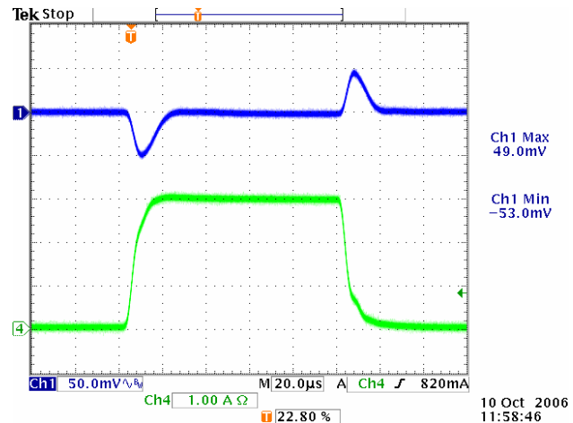
Load transient, 0 – 3A, V IN /V OUT = 5.5V/3.3V
