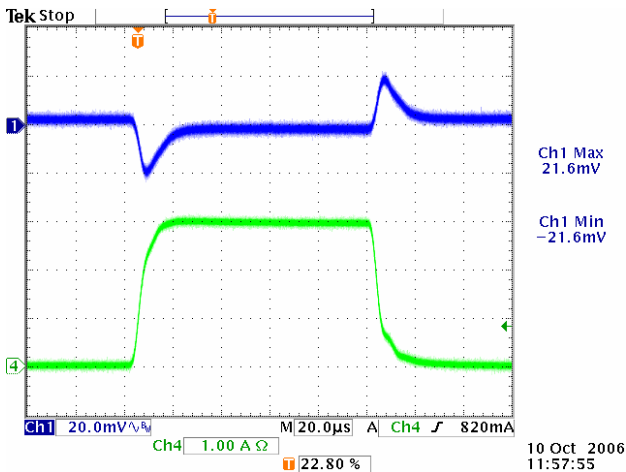
Load transient, 0 – 3A, V IN /V OUT = 5.5V/1.2V
