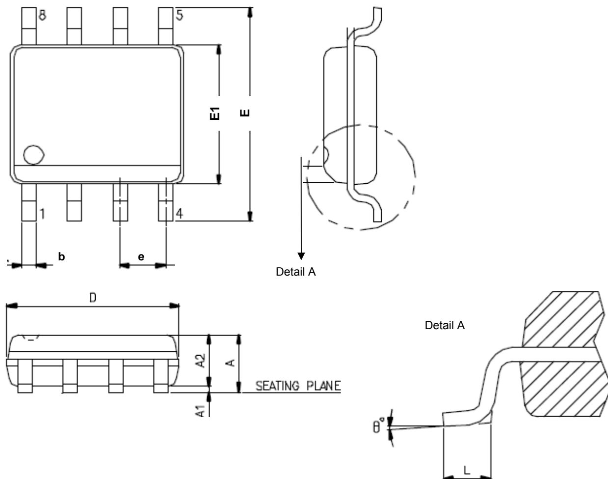
Figure 28. SOP 8 ( 150 mil )
