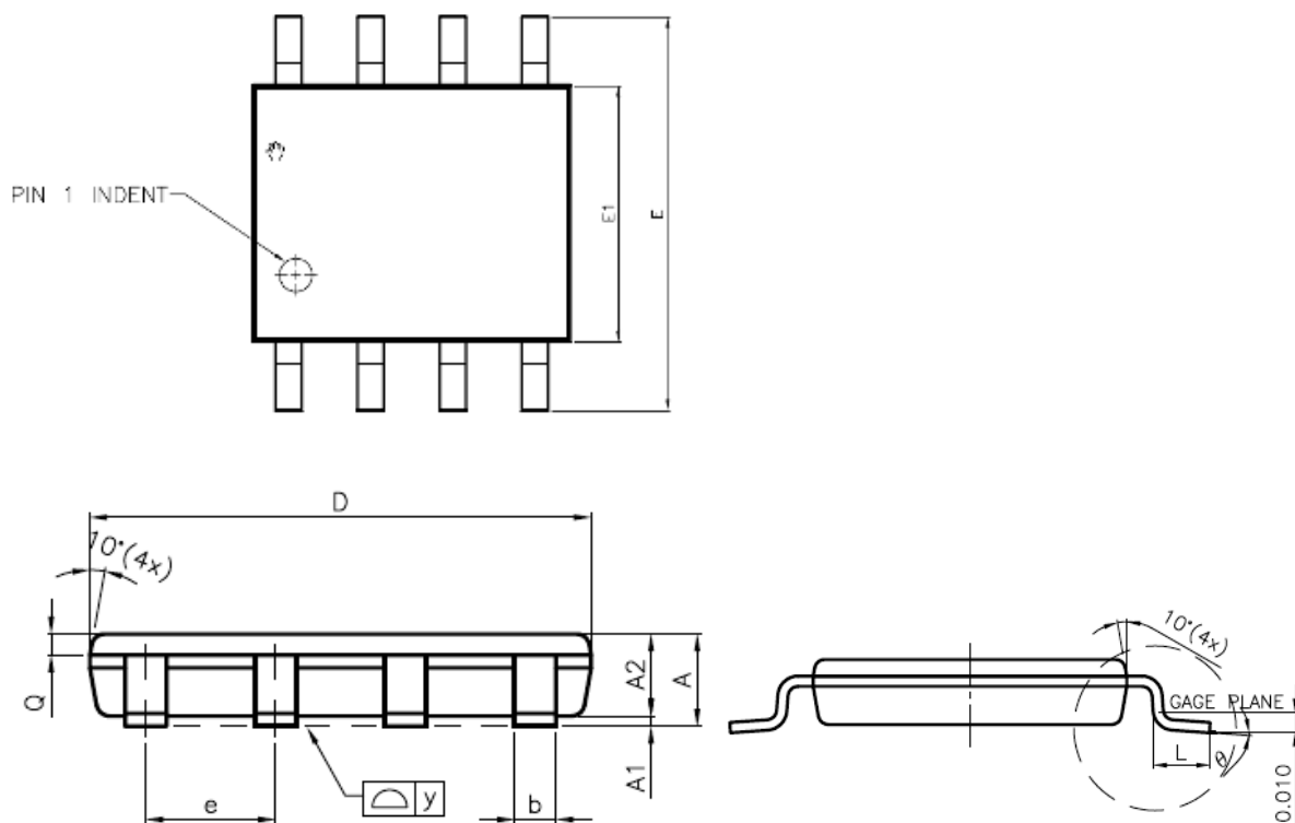
Figure 47. VSOP 8 ( 150 mil )
