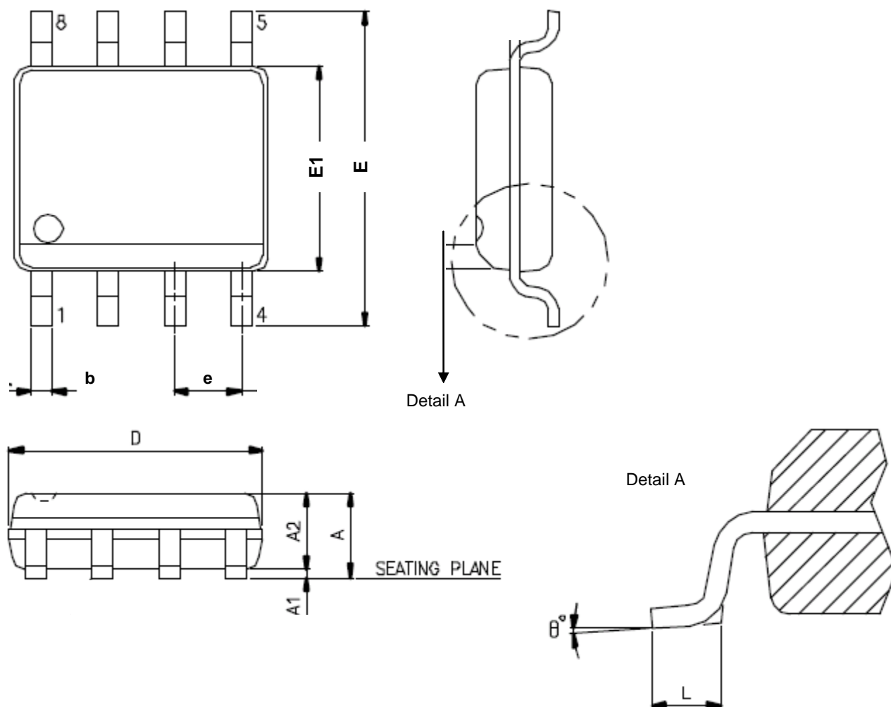
Figure 45. SOP 8 ( 150 mil )
