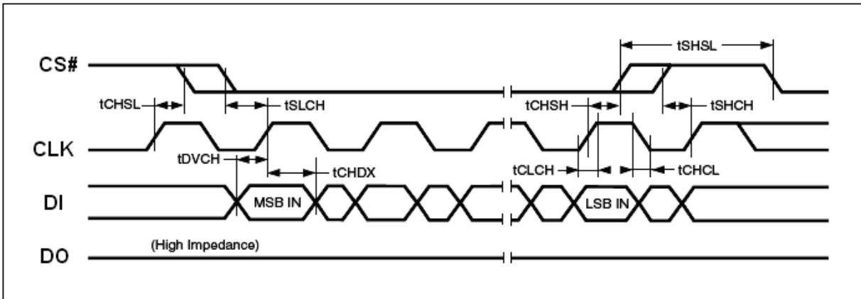
Figure 43. Input Timing
