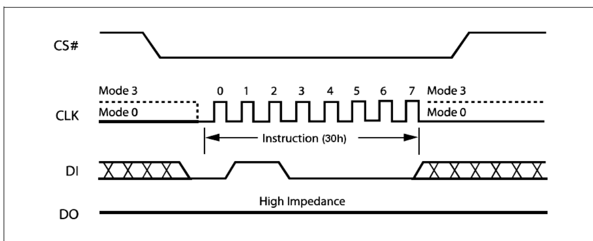
Figure 26. Write Resume Instruction Sequence Diagram
