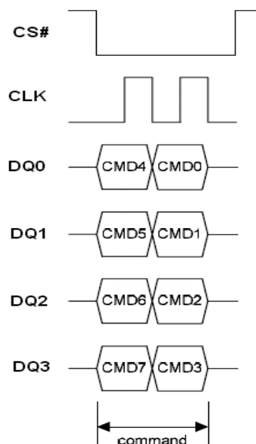
Figure 26.1 Write Suspend/Resume Instruction Sequence in QPI Mode
