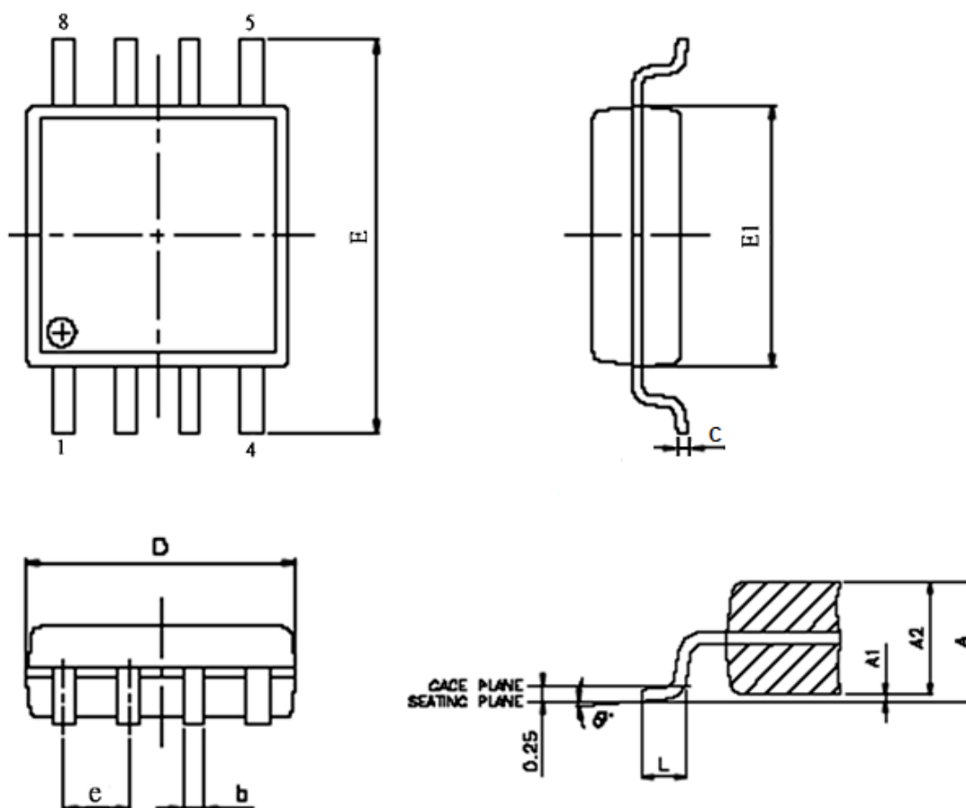
Figure 46. SOP 200 mil ( official name = 208 mil )
