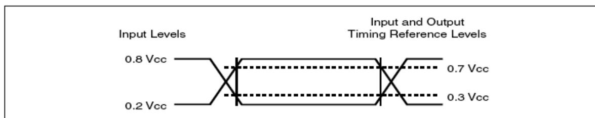
Figure 41. AC Measurement I/O Waveform
