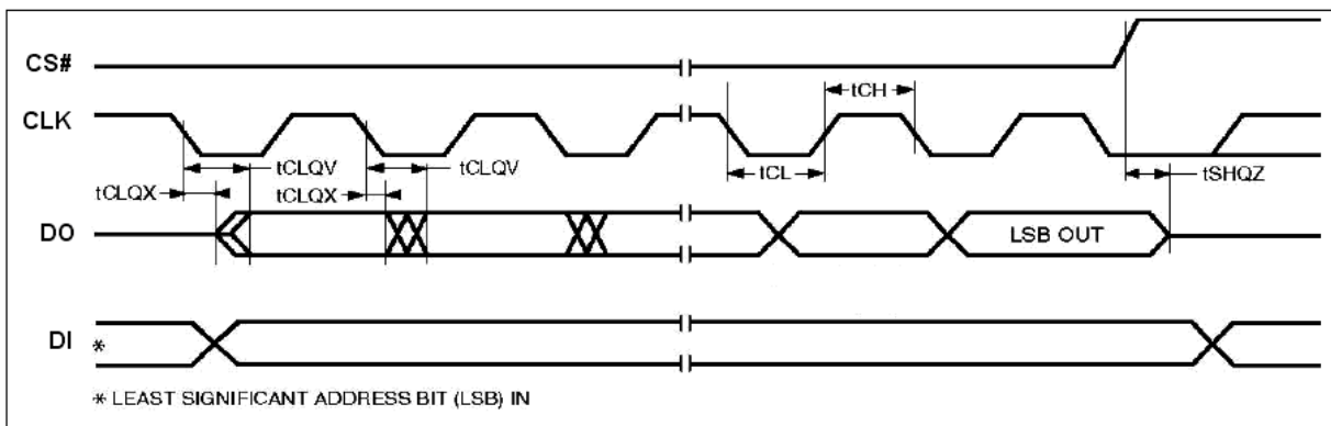
Figure 42. Serial Output Timing
