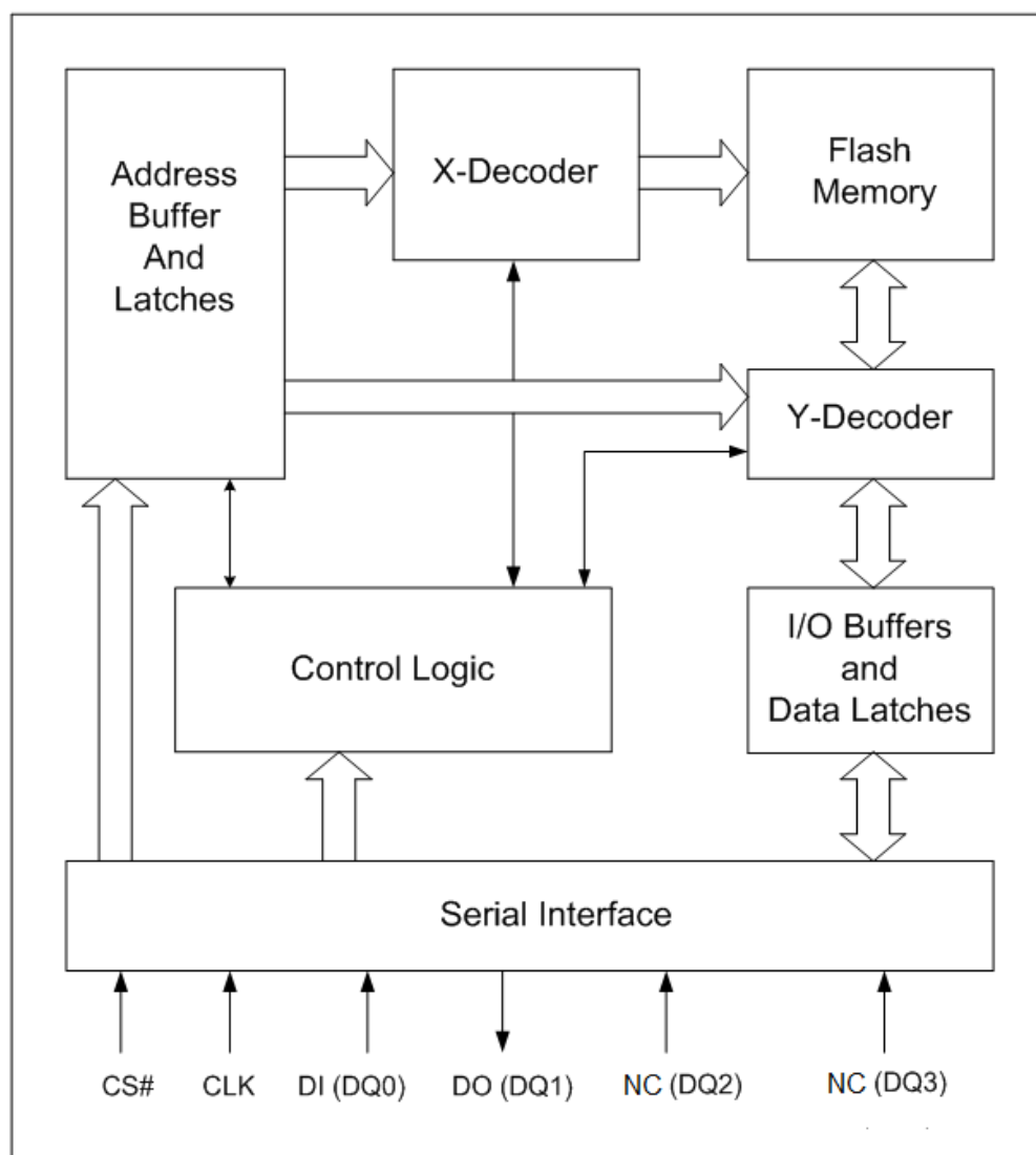
Figure 2. BLOCK DIAGRAM
