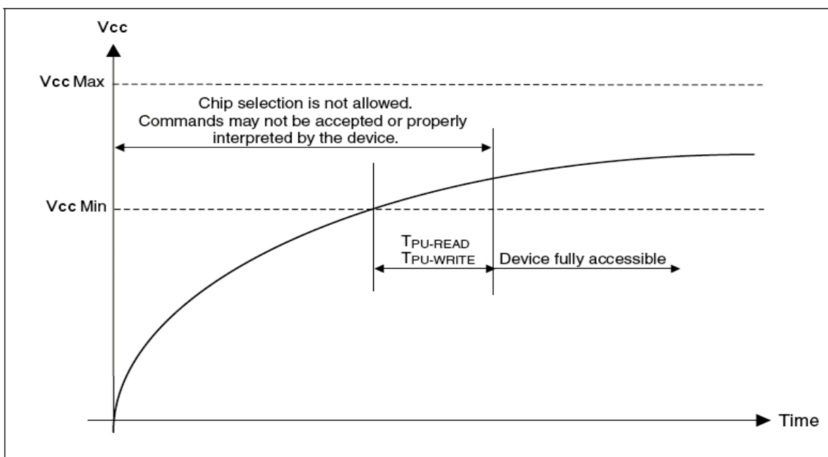
Figure 40. Power-up Timing
