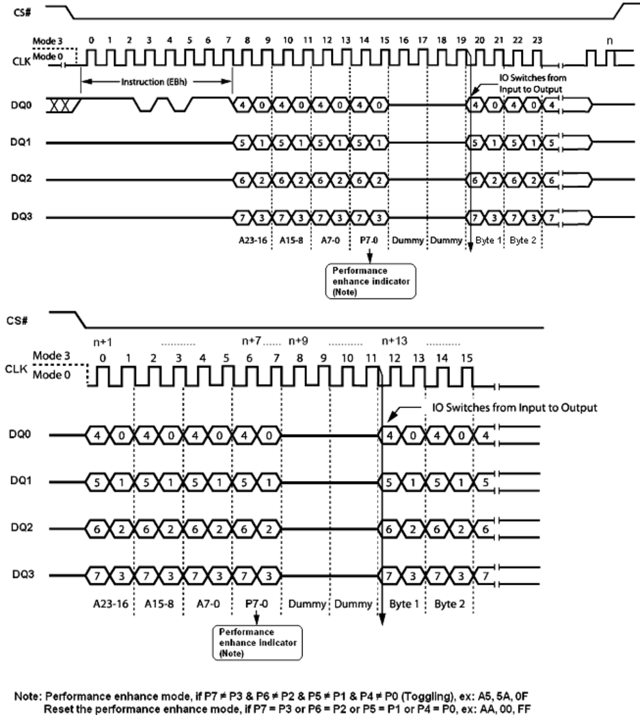
Figure 20. Quad Input/Output Fast Read Enhance Performance Mode Sequence Diagram
