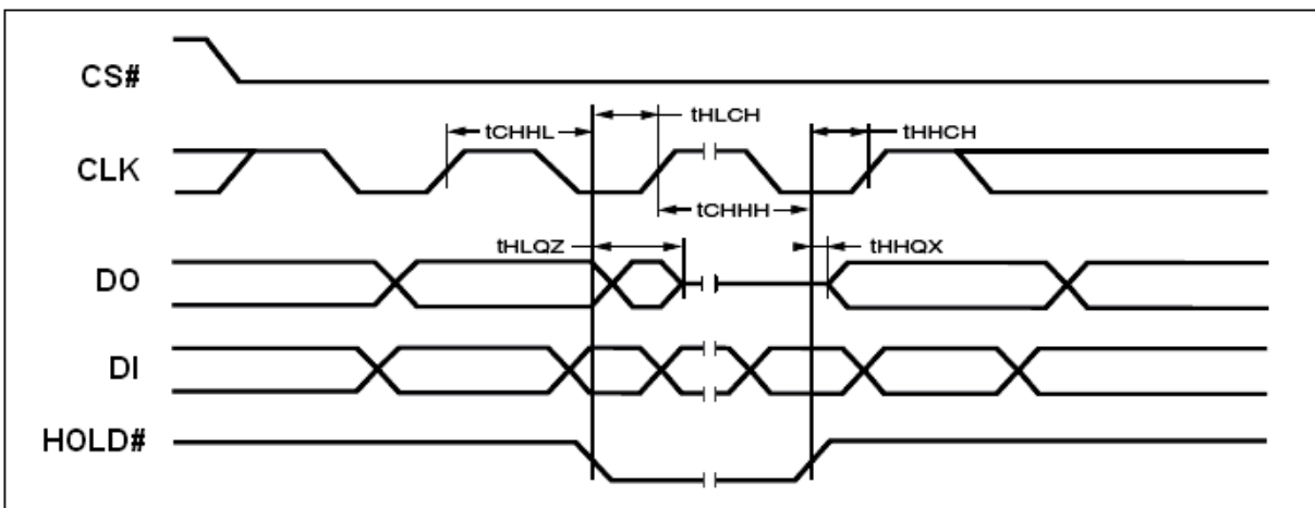
Figure 44. Hold Timing
