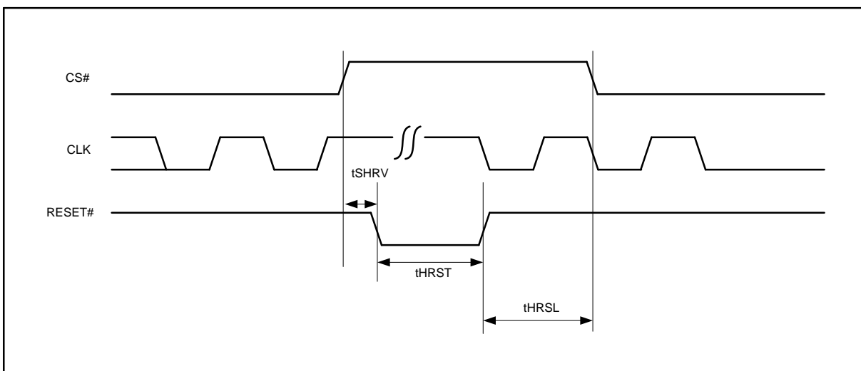
Figure 45. Reset Timing
