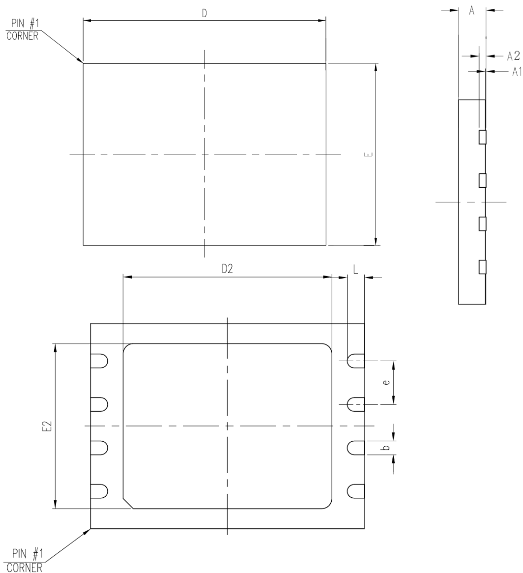
Figure 48. VDFN8 ( 5x6mm )
