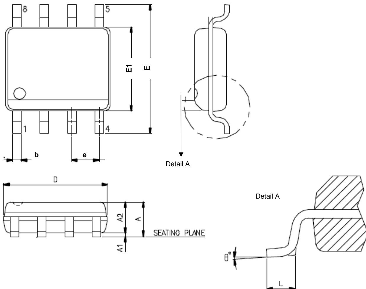
Figure 28. SOP 8 ( 150 mil )
