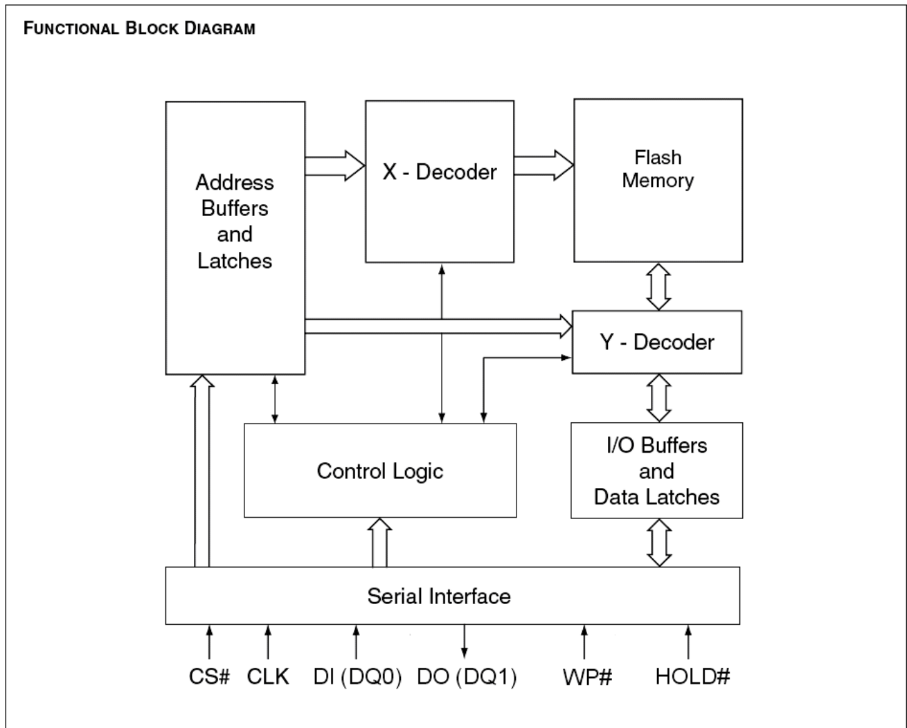
Figure 2. BLOCK DIAGRAM
