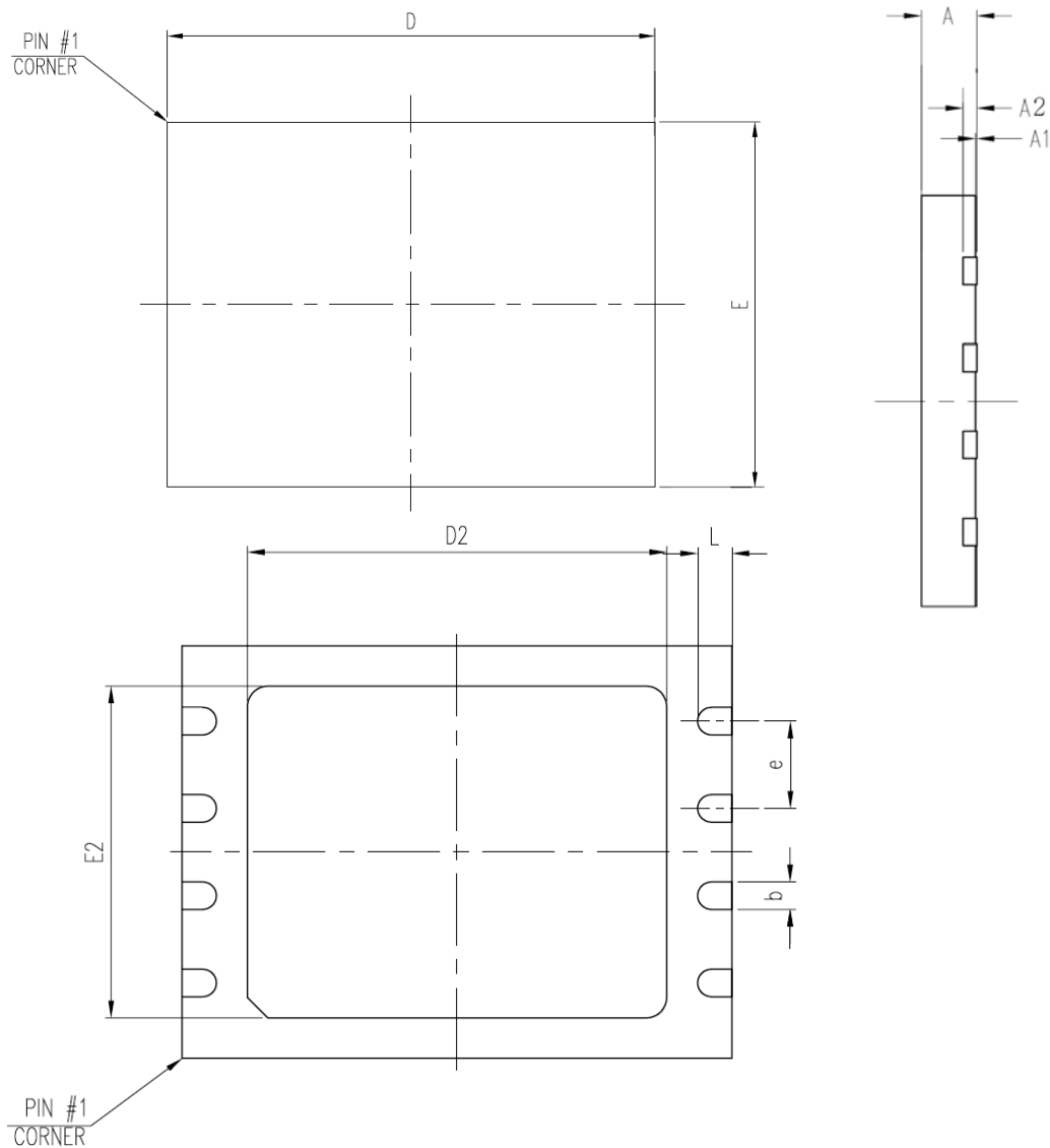
Figure 30. VDFN8 ( 5x6mm )
