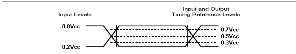
Figure 39. AC Measurement I/O Waveform
