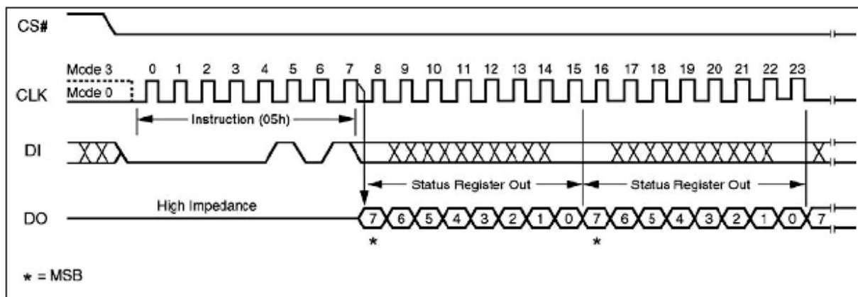
Figure 10. Read Status Register Instruction Sequence Diagram
