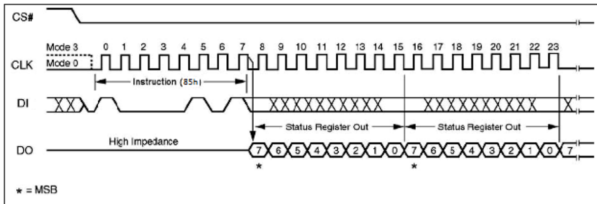
Figure 14. Read Status Register 4 Instruction Sequence Diagram
