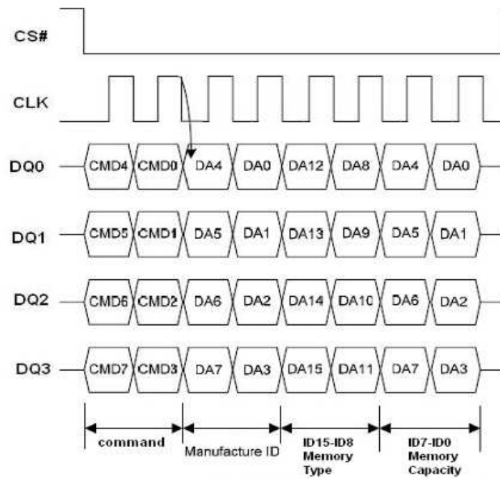
Figure 39.1 Read Identification (RDID) in QPI Mode
