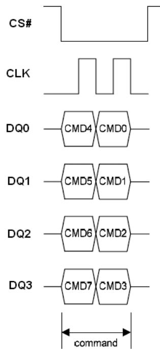
Figure 40.1 Enter OTP Mode Sequence in QPI Mode
