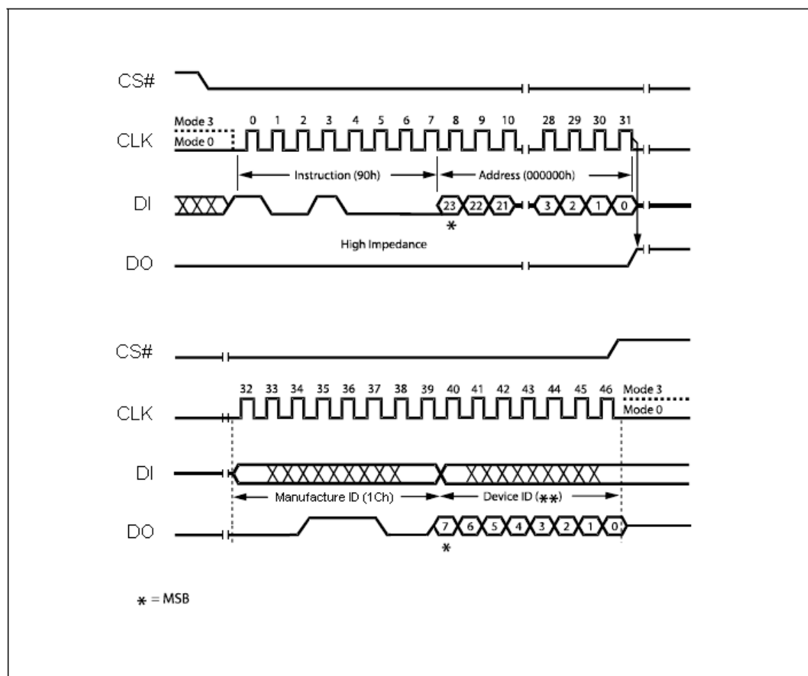
Figure 38. Read Manufacturer / Device ID Diagram
