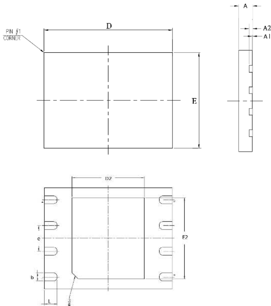
Figure 50. VDFN8 ( 5x6mm )
