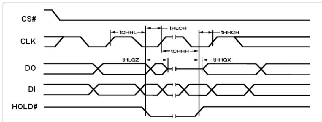
Figure 46. Hold Timing
