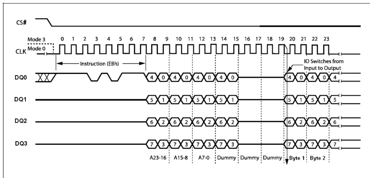
Figure 4. Quad I/O SPI Modes
