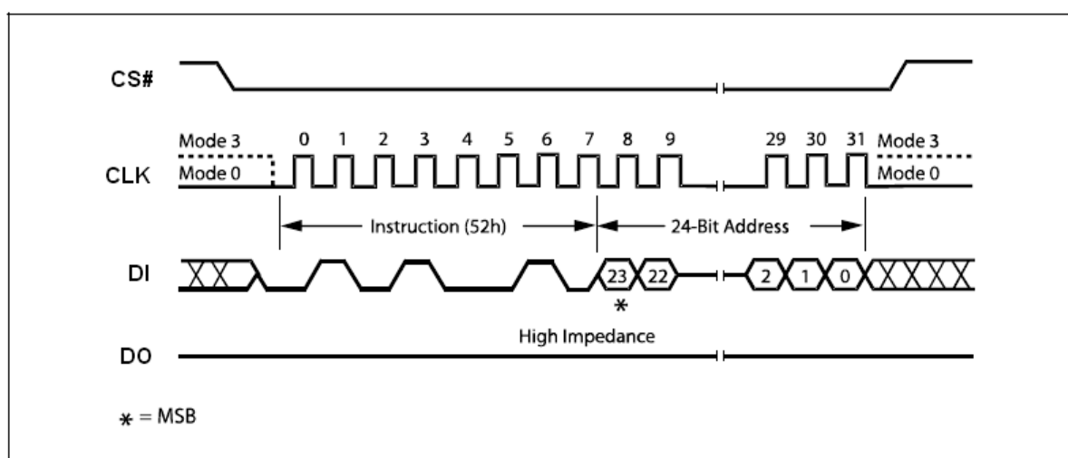
Figure 32. 32KB Half Block Erase Instruction Sequence Diagram
