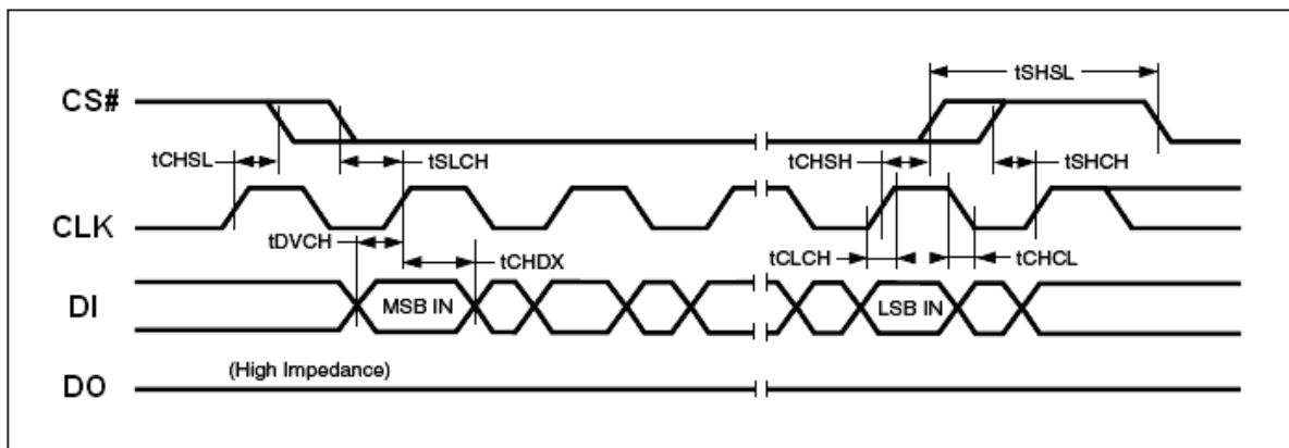
Figure 45. Input Timing
