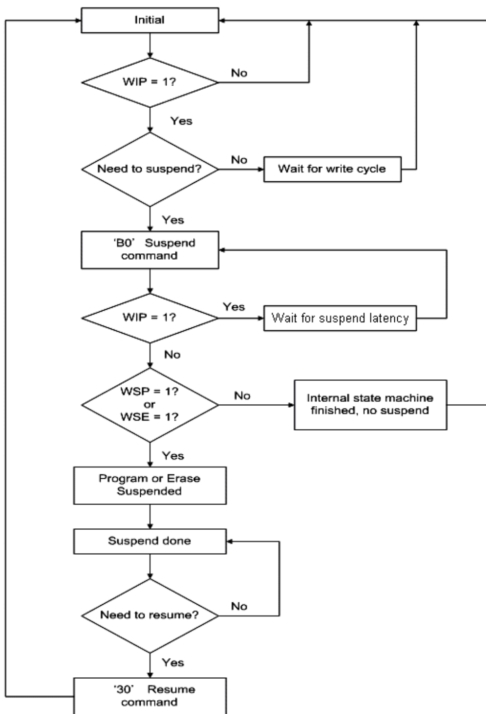
Figure 30. Write Suspend/Resume Flow
