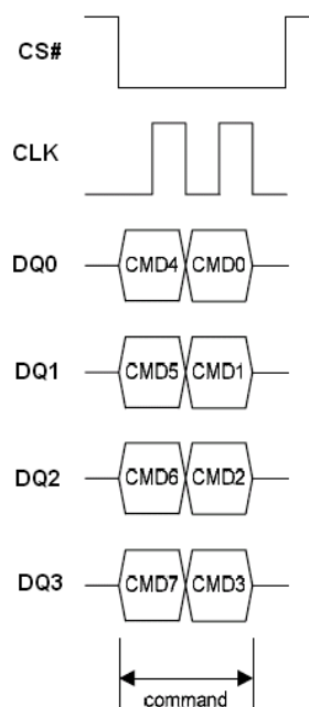
Figure 10.1 Write Enable/Disable Instruction Sequence under QPI Mode
