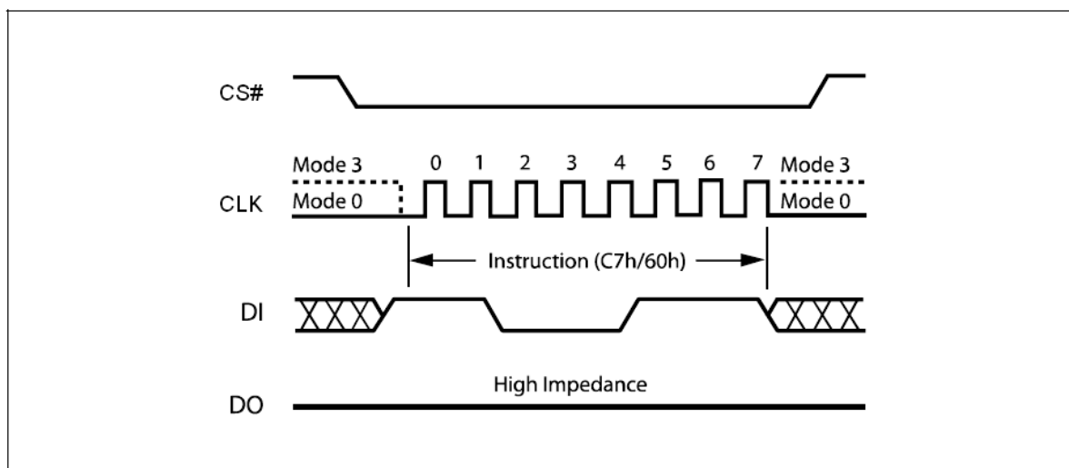
Figure 34. Chip Erase Instruction Sequence Diagram
