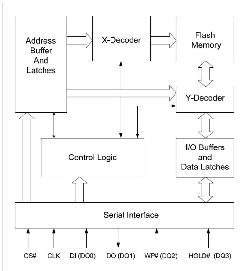
Figure 2. BLOCK DIAGRAM
