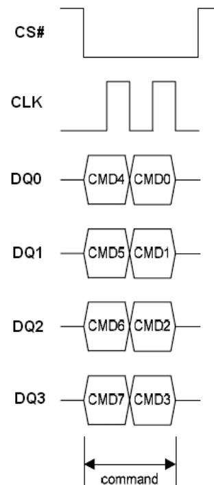
Figure 34.1 Chip Erase Sequence under EQPI Mode
