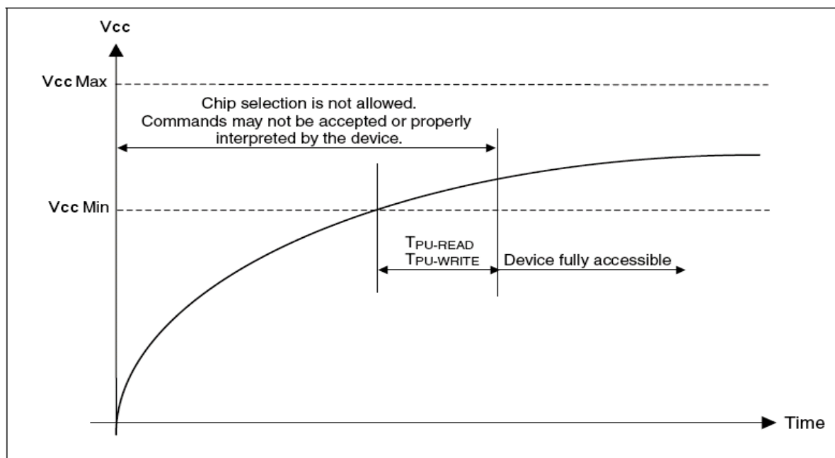
Figure 42. Power-up Timing
