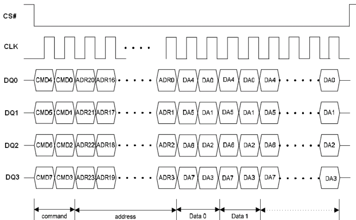
Figure 25.1 Program Instruction Sequence in QPI Mode
