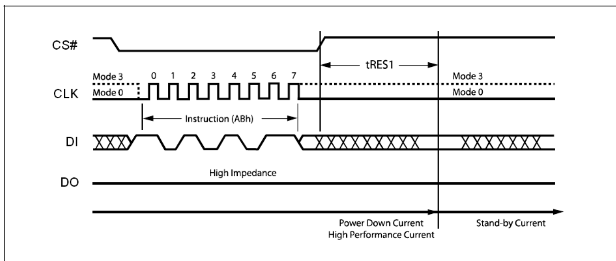
Figure 36. Release Power-down Instruction Sequence Diagram
