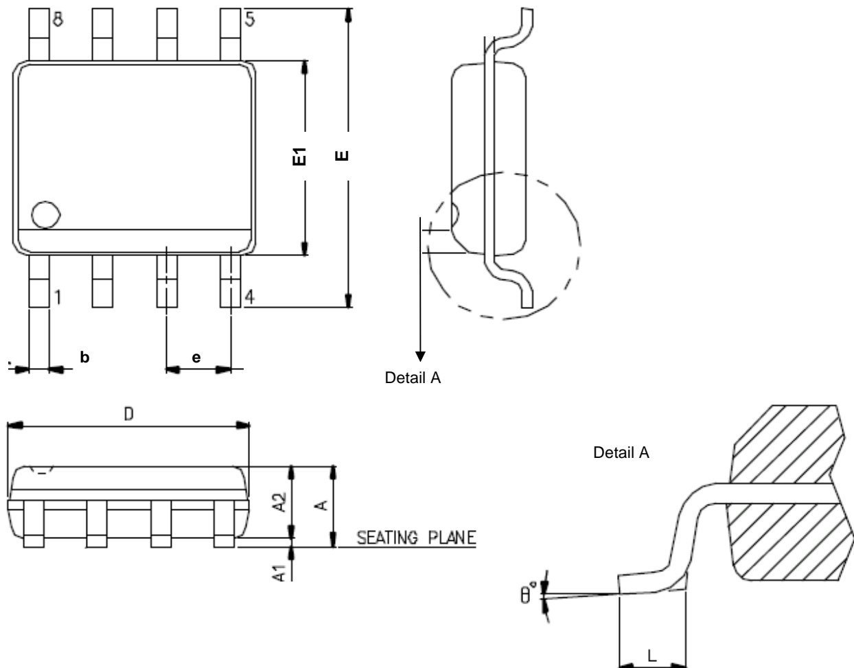
Figure 47. SOP 8 ( 150 mil )
