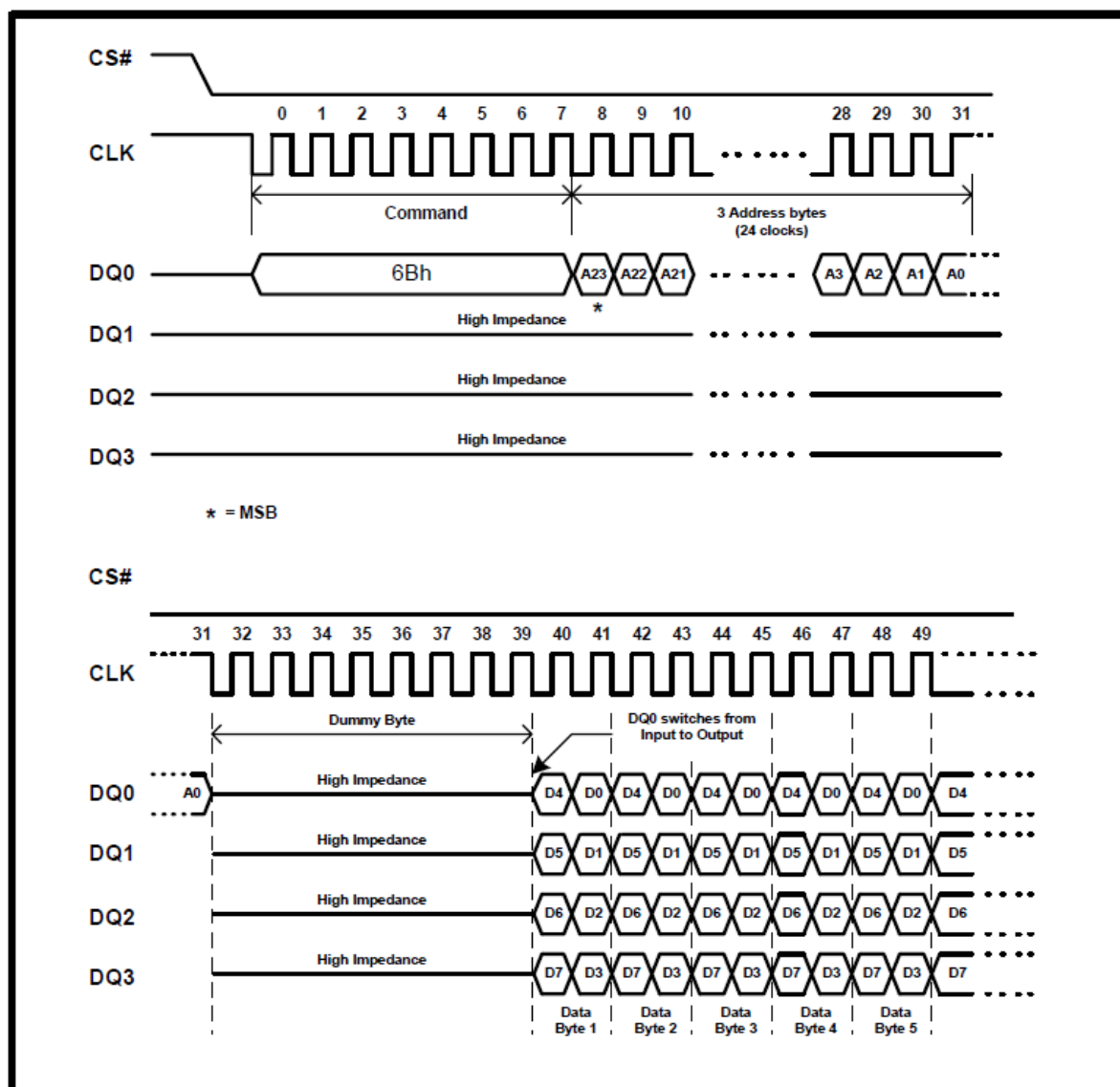
Figure 20. Quad Output Fast Read Instruction Sequence Diagram
