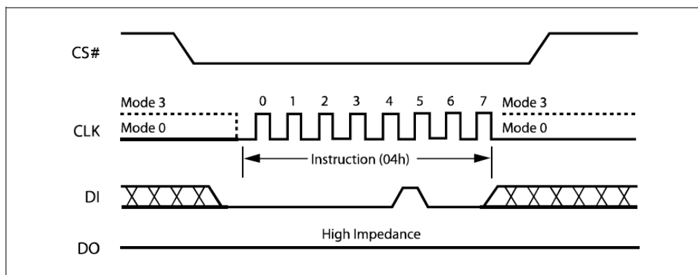
Figure 10. Write Disable Instruction Sequence Diagram
