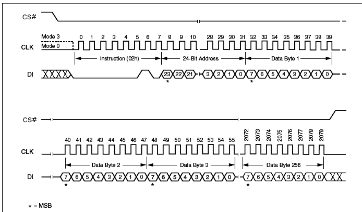
Figure 25. Page Program Instruction Sequence Diagram
