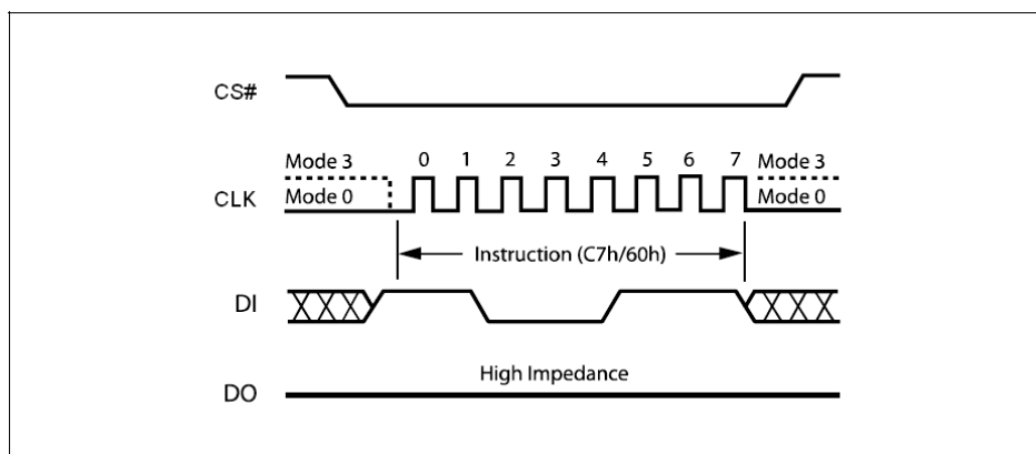
Figure 31. Chip Erase Instruction Sequence Diagram
