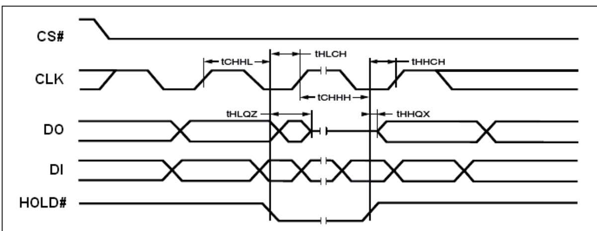
Figure 43. Hold Timing
