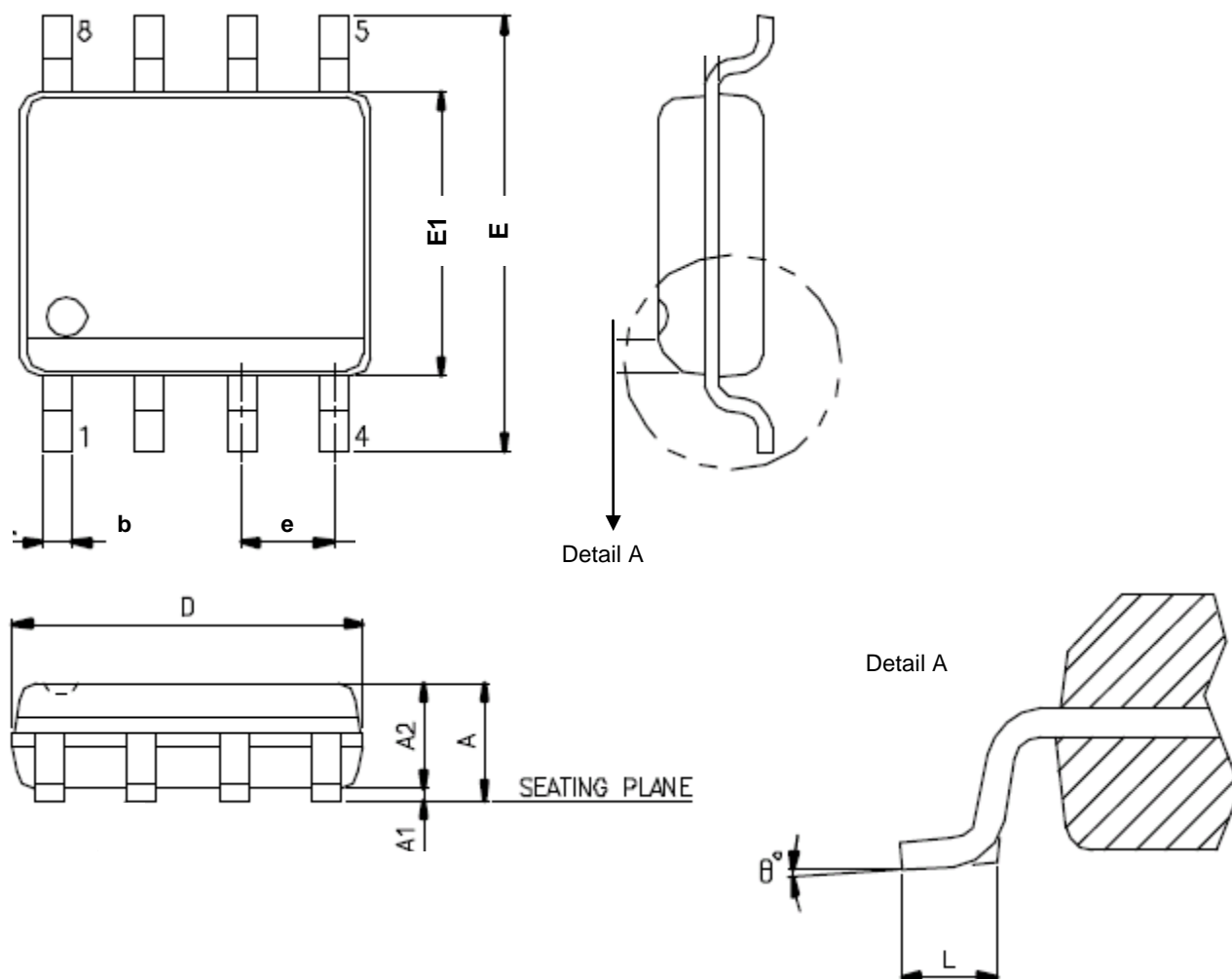
Figure 44. SOP 8 ( 150 mil )
