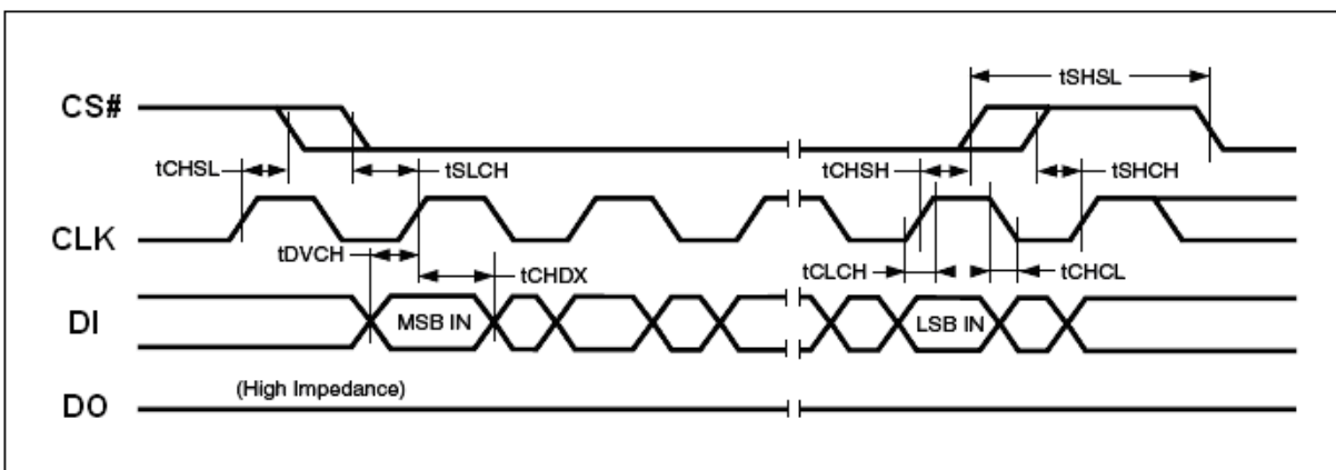
Figure 42. Input Timing
