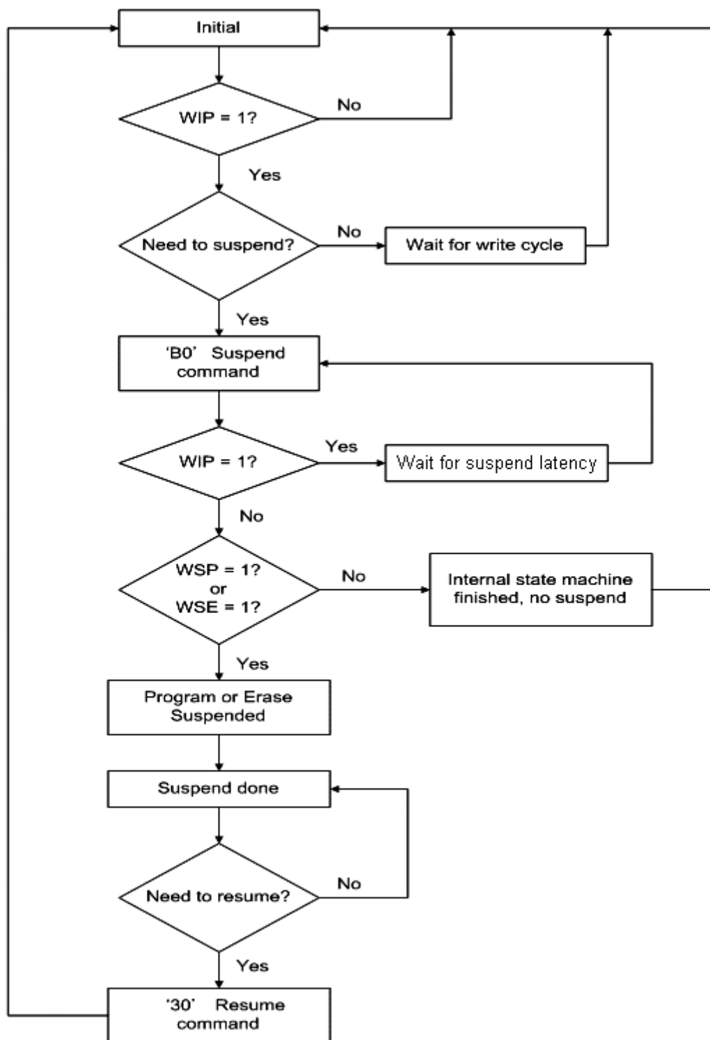
Figure 28. Write Suspend/Resume Flow
