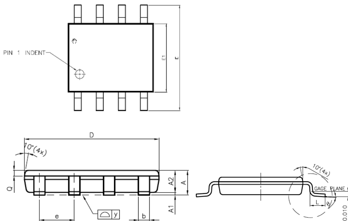
Figure 47. VSOP 8 ( 150 mil )
