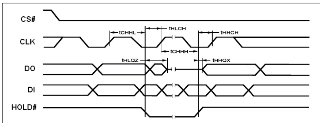
Figure 44. Hold Timing
