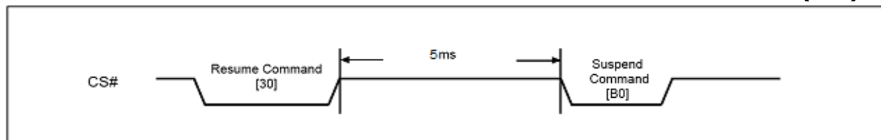
Figure 26.3 Resume to Suspend Latency
