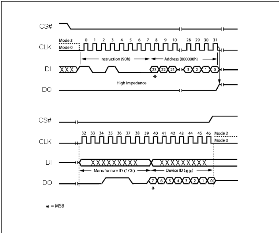
Figure 36. Read Manufacturer / Device ID Diagram
