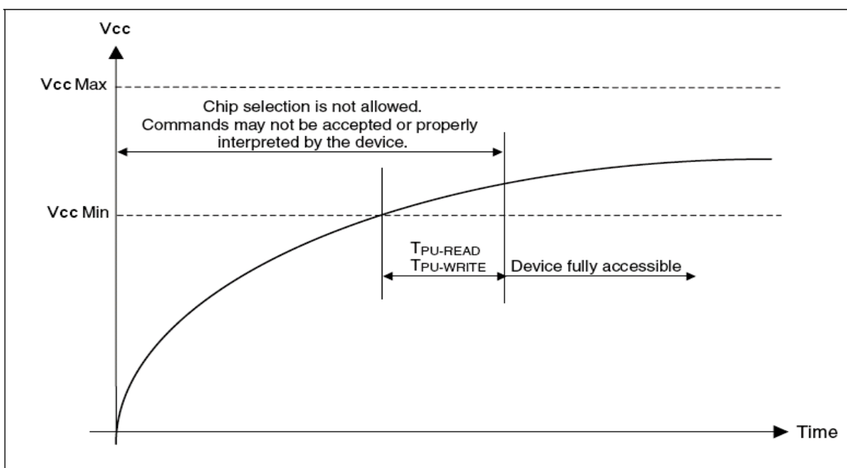
Figure 39. Power-up Timing
