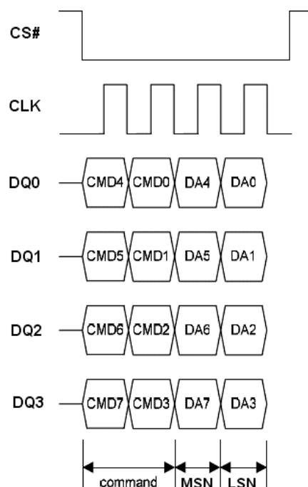
Figure 23. Write Status Register 2 Instruction Sequence Diagram
