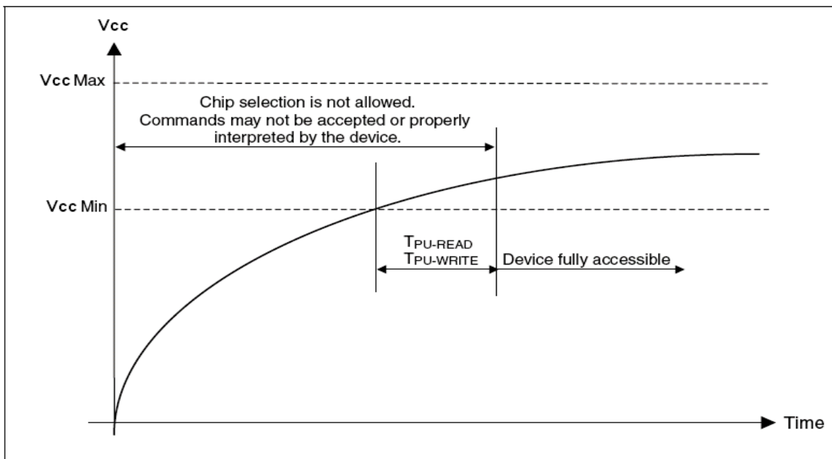
Figure 39. Power-up Timing
