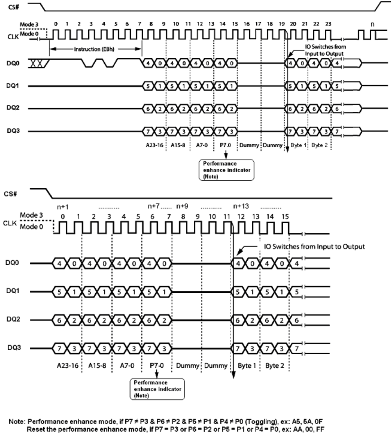
Figure 21. Quad Input/Output Fast Read Enhance Performance Mode Sequence Diagram
