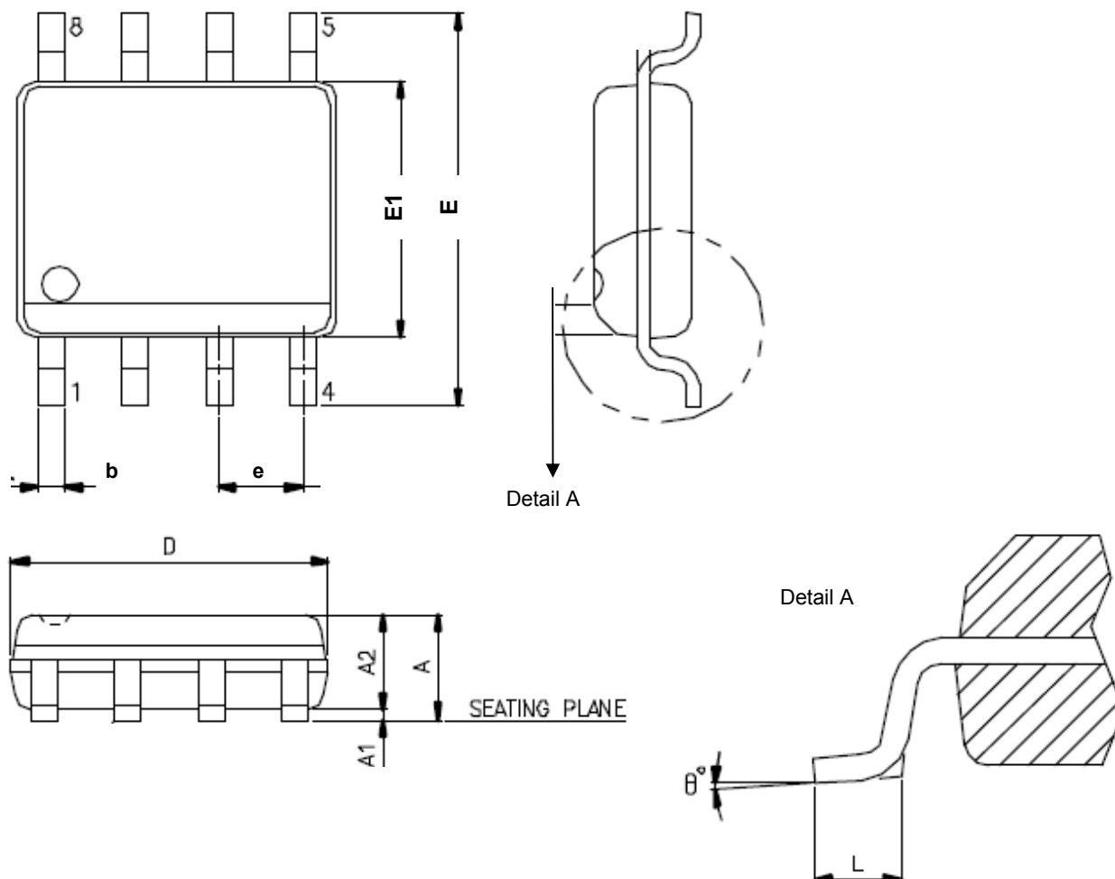
Figure 28. SOP 8 ( 150 mil )
