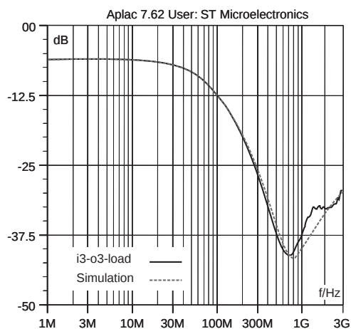
Fig. 3: Digital crosstalk measurements.
