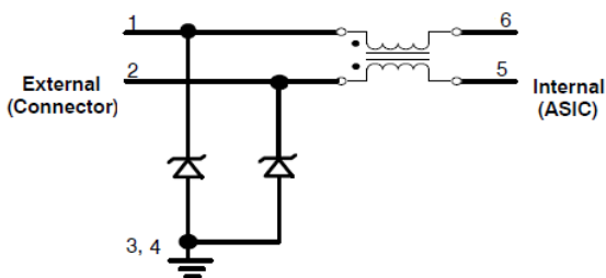
Figure 1. EMI8131 Electrical Schematic
