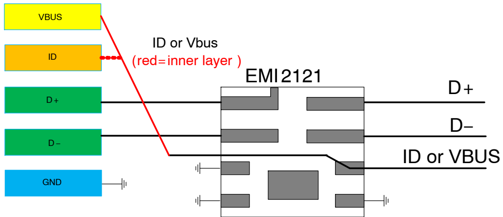
Figure 15. EMI2121 Micro – USB Connector Application Diagram
