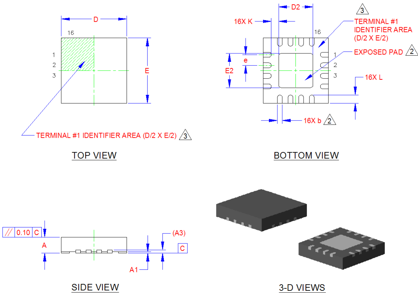
Figure 7.5 16-Pin QFN 4mm x 4mm Package Drawing
