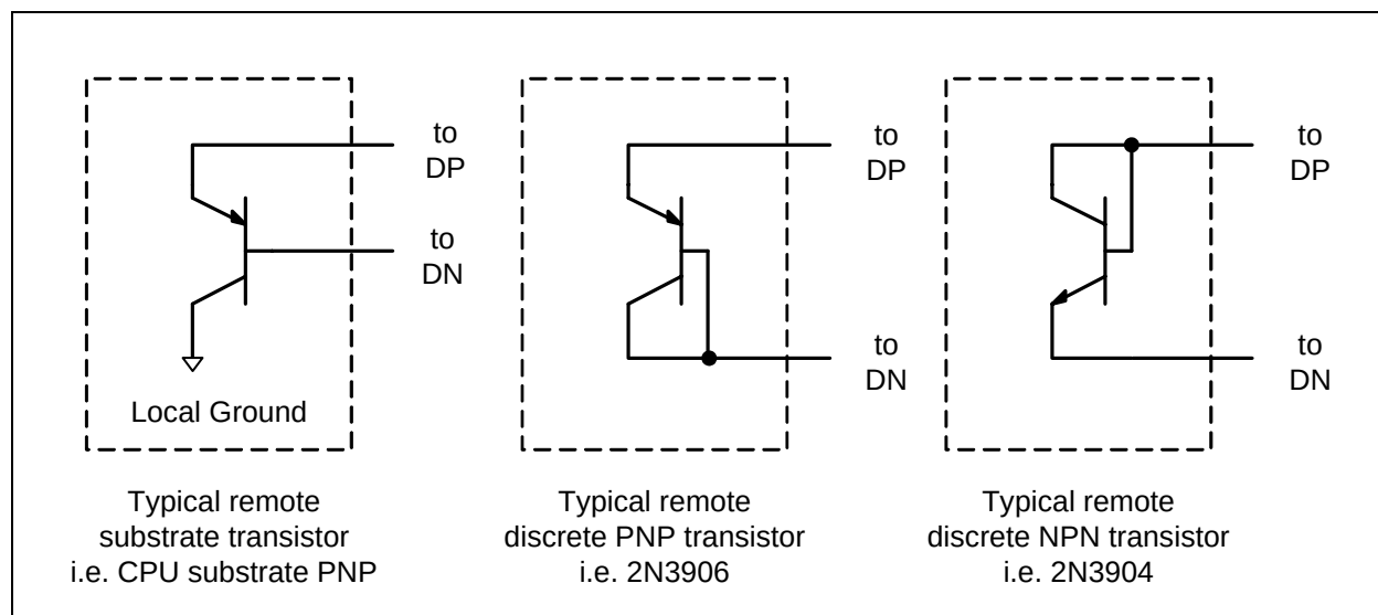
Figure 4.4 Diode Connections
