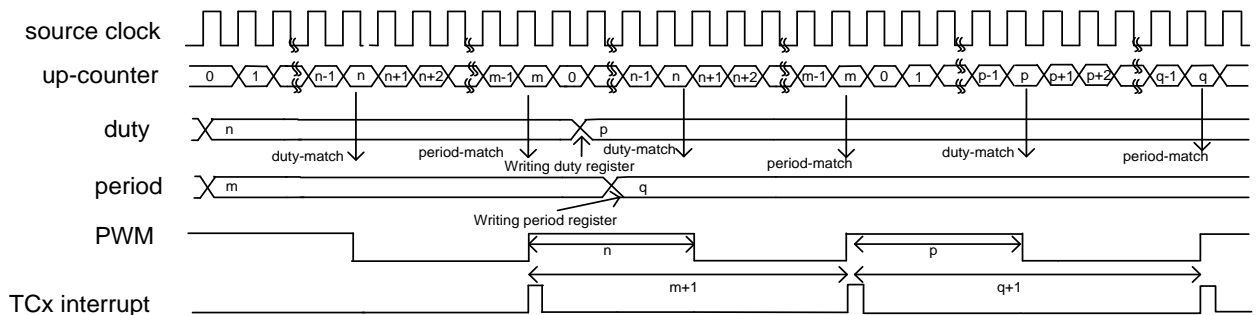
Figure 6-22 PWM Mode Waveform
