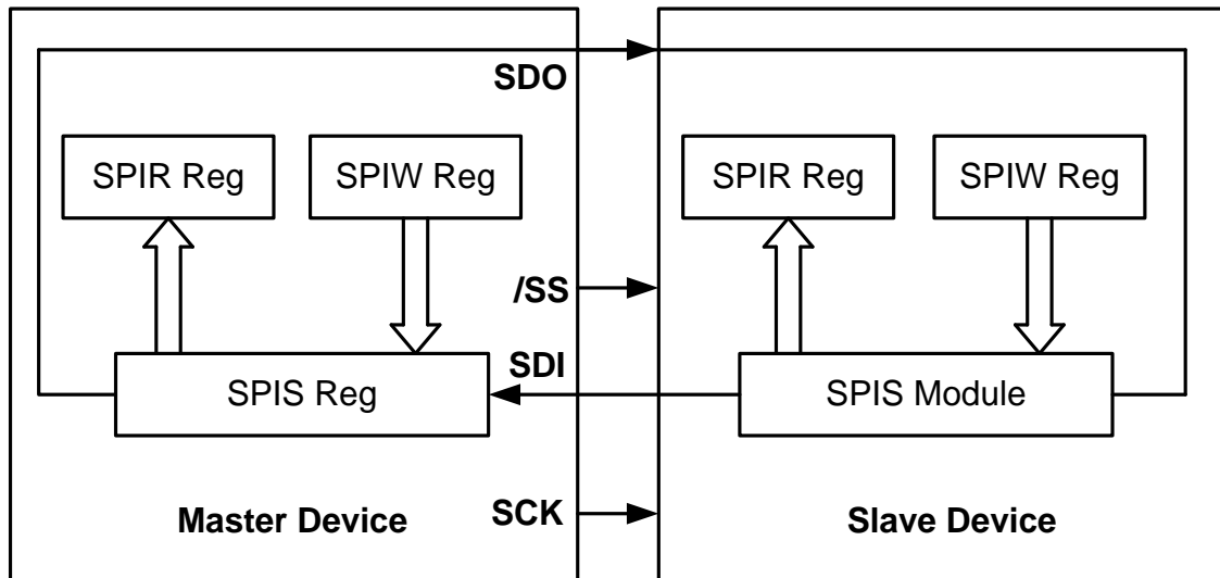
Figure 6-30 SPI Master/Slave Communication
