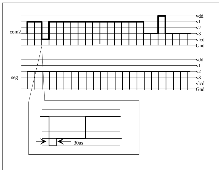
Fig.11 key scan signal
