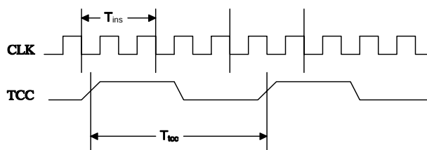
Fig.18 AC timing
