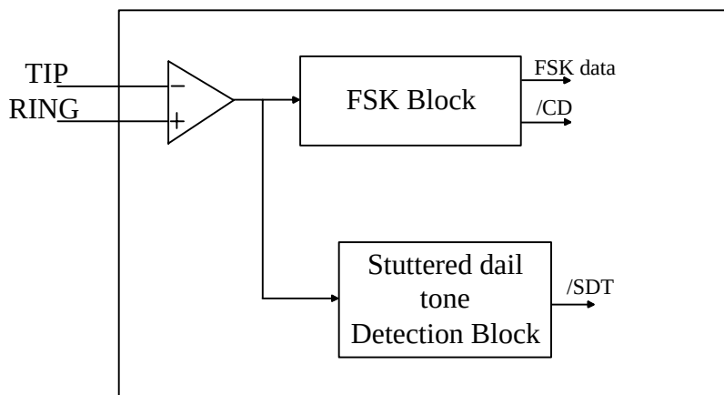
Fig.17 Stuttered dial tone block diagram
