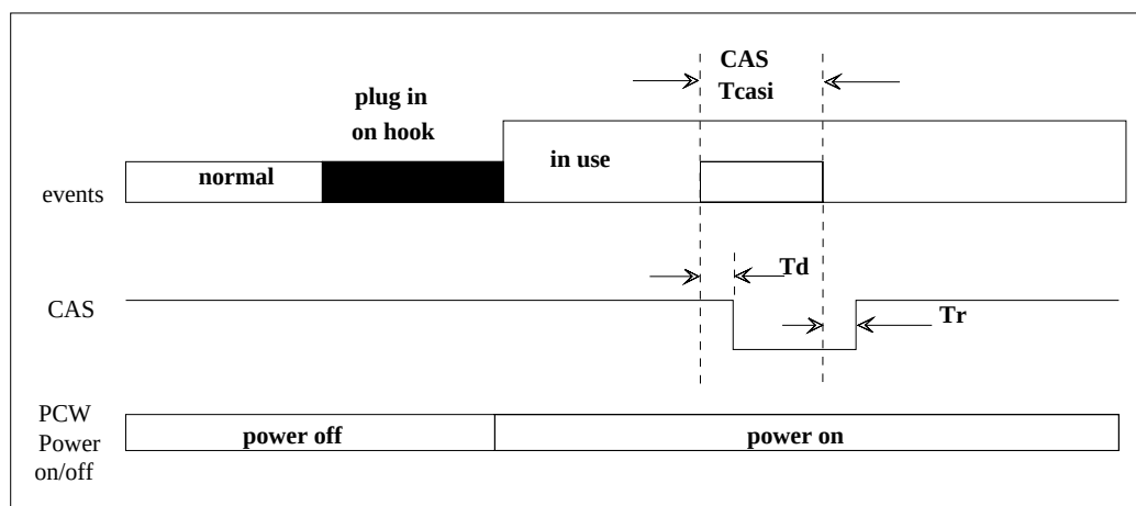
Fig.20 Call Waiting Timing Diagram
