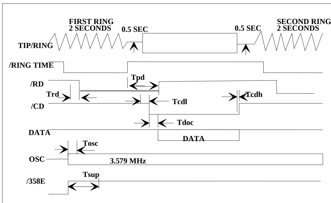
Fig.19 FSK Timing Diagram
