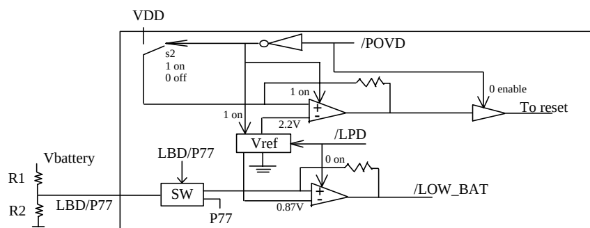
Fig.7 Universal low battery detect with /LPD,/POVD and /LOW_BAT
