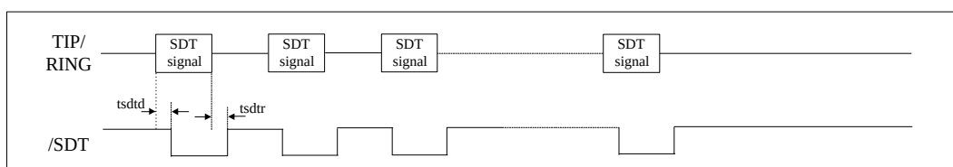
Fig.21 Stuttered dial tone detect. timing diagram
