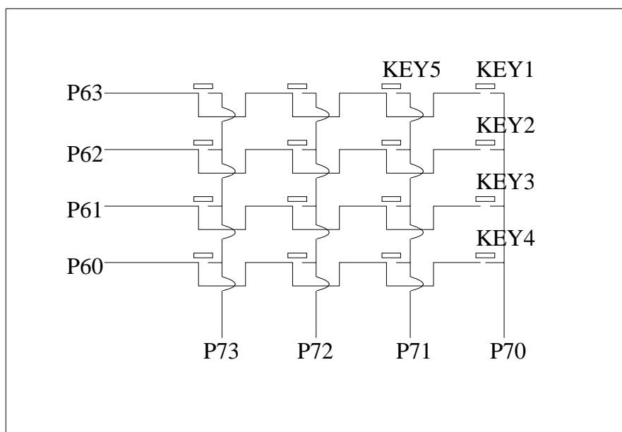
Fig.10. Key scan circuit
