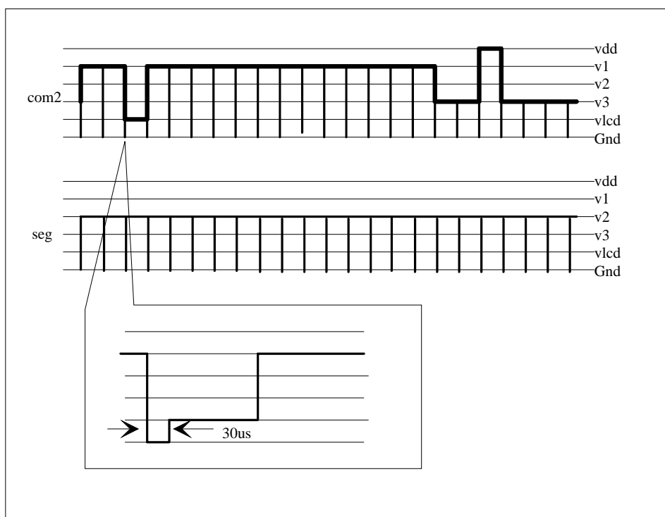
Fig.11.key scan signal
