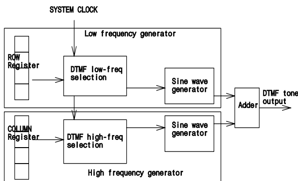
Fig17. DTMF Block Diagram
