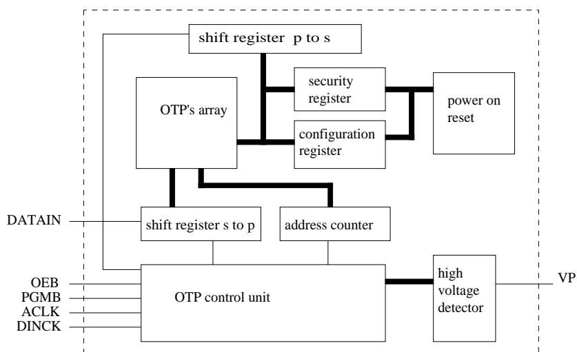
Fig2. Block diagram1
