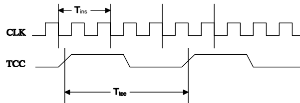
Fig.22 AC timing
