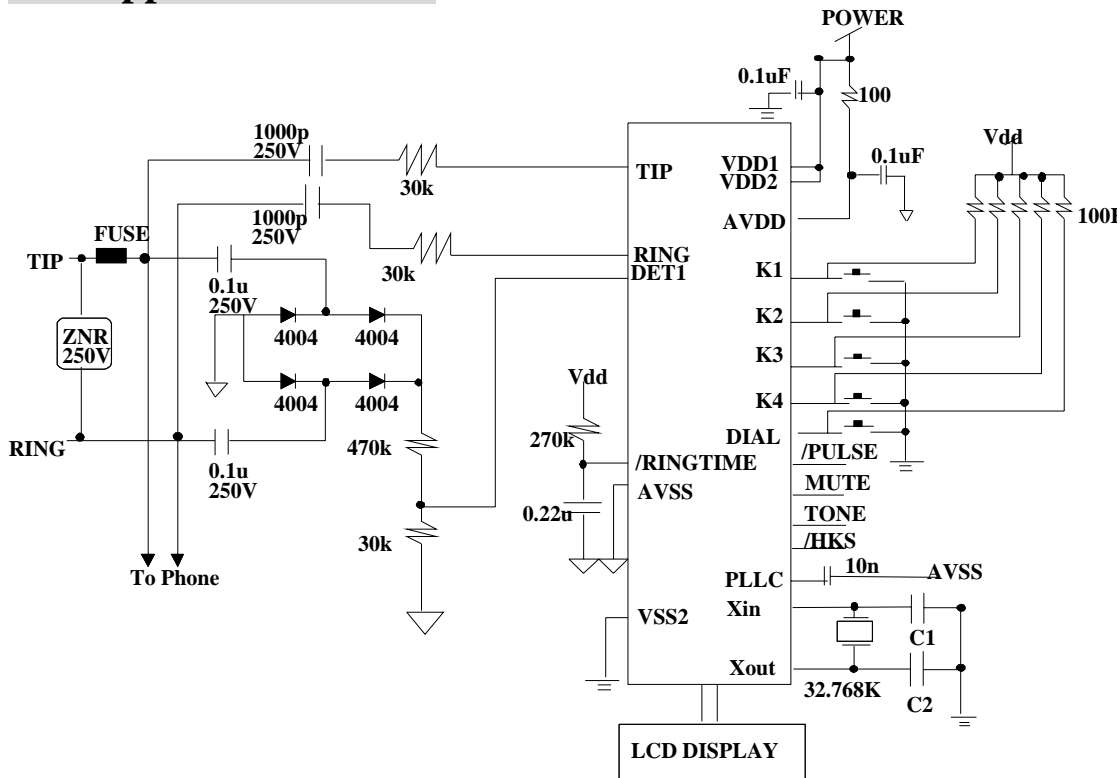
Fig.24.application circuit
