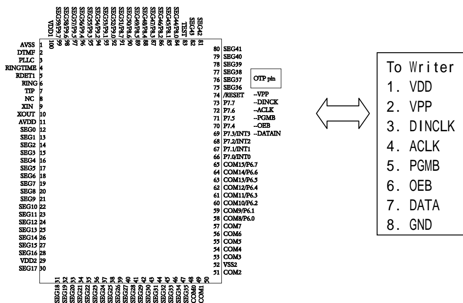
Fig1. Pin Assignment
