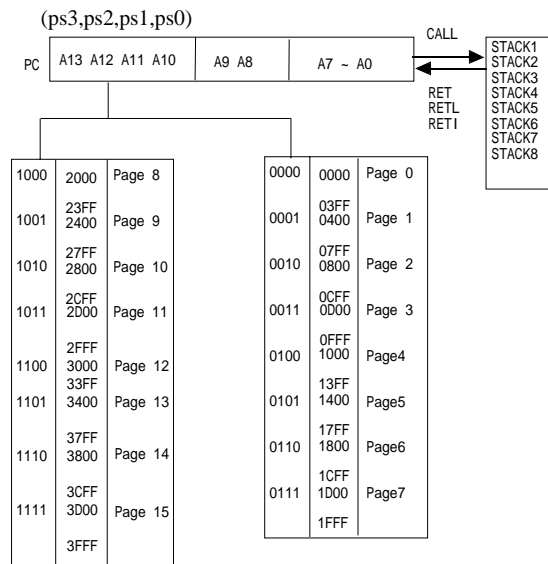
Fig.4 Program counter organization
