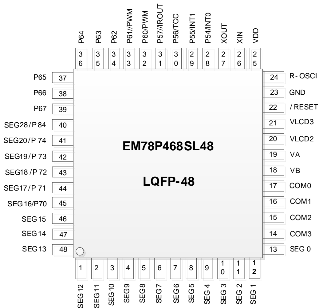
Figure 3-3 48-Pin LQFP/QFP EM78P468SL48 Pin Assignment
