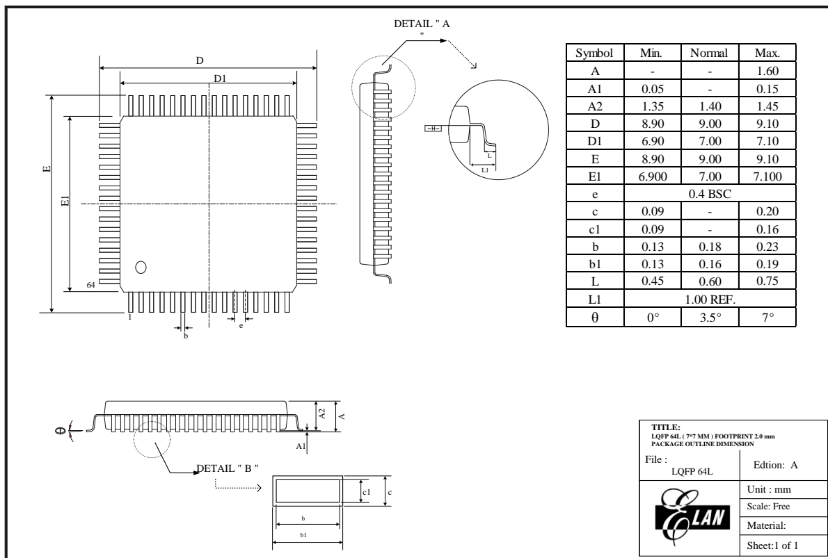
Figure C-1c EM78P468S LQFP-64L Package Type
