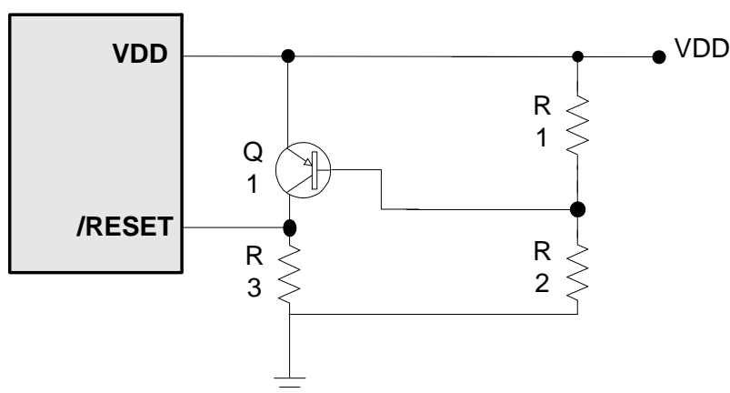
Figure 6-12 Residue Voltage Protection Circuit 2
