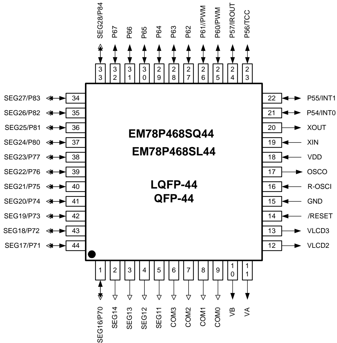
Figure 3-4 44-Pin LQFP/QFP EM78P468SQ44/EM78P468SL44 Pin Assignment
