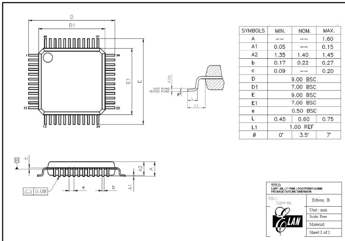
Figure C-1f EM78P468S LQFP-48L Package Type
