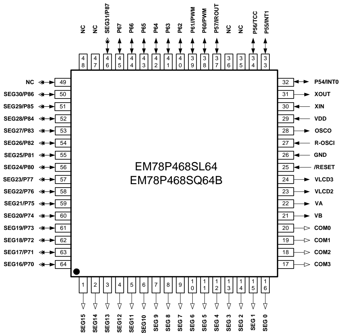
Figure 3-2 64-Pin LQFP/QFP EM78P468SL64/EM78P468SQ64B Pin Assignment
