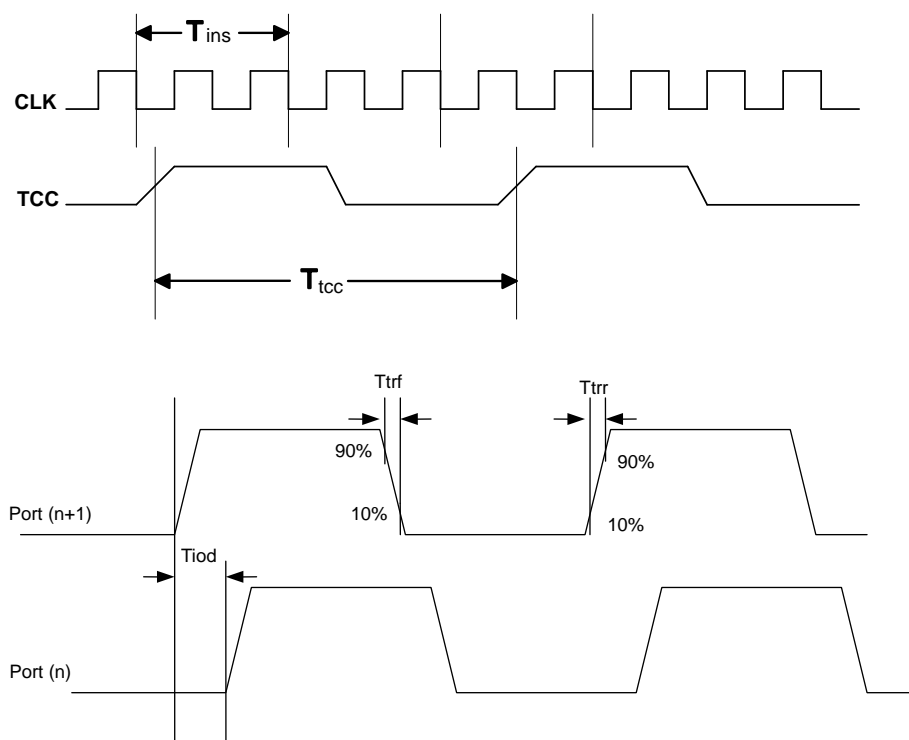
Figure 6-27 Timing Diagrams of EM78P468S
