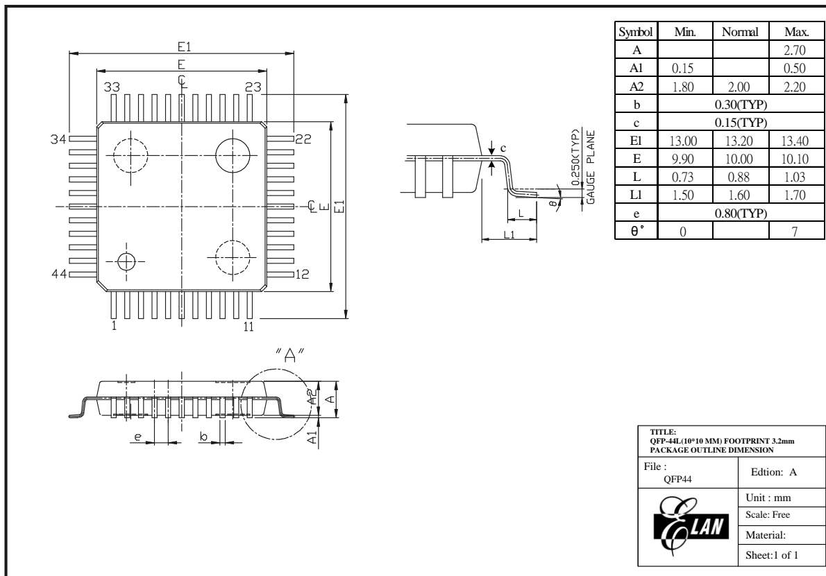
Figure C-1e EM78P468S QFP-44 Package Type
