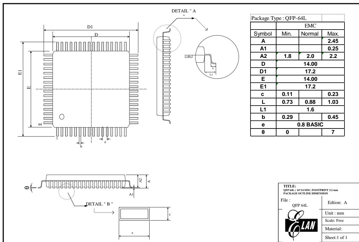
Figure C-1b EM78P468S QFP-64L Package Type
