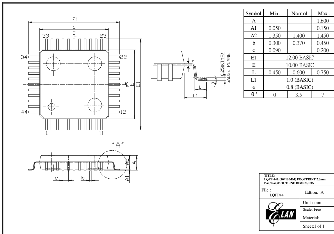
Figure C-1d EM78P468S LQFP-44 Package Type
