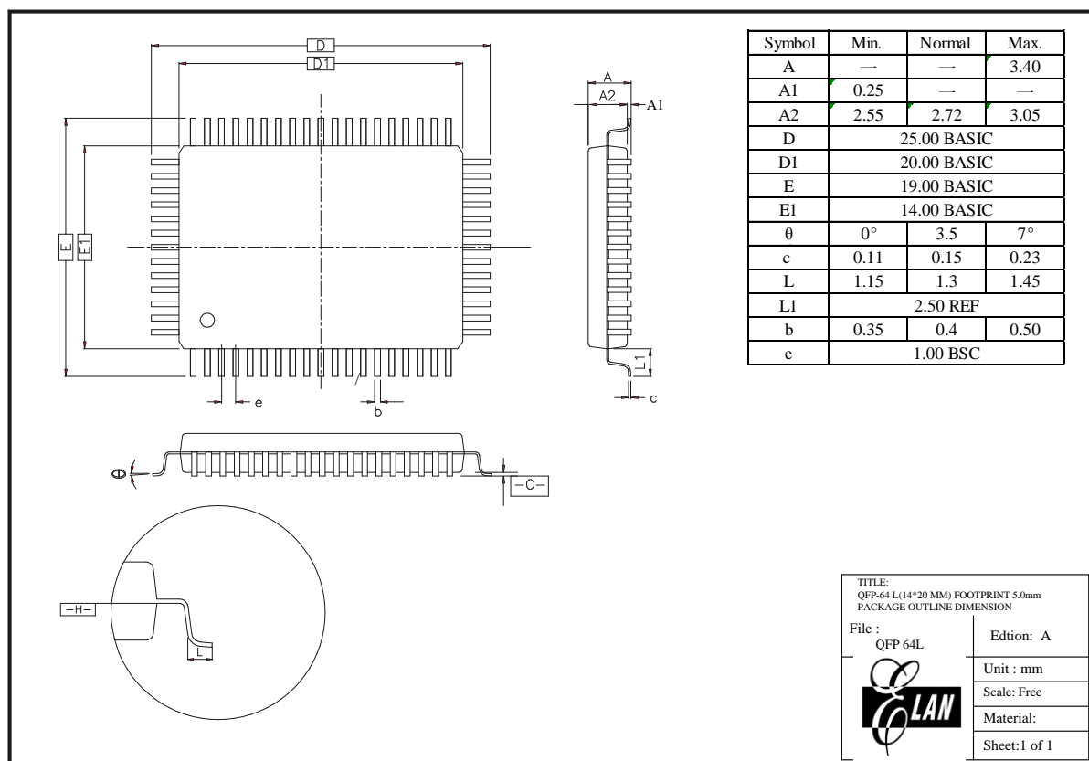
Figure C-1a EM78P468S QFP-64L Package Type
