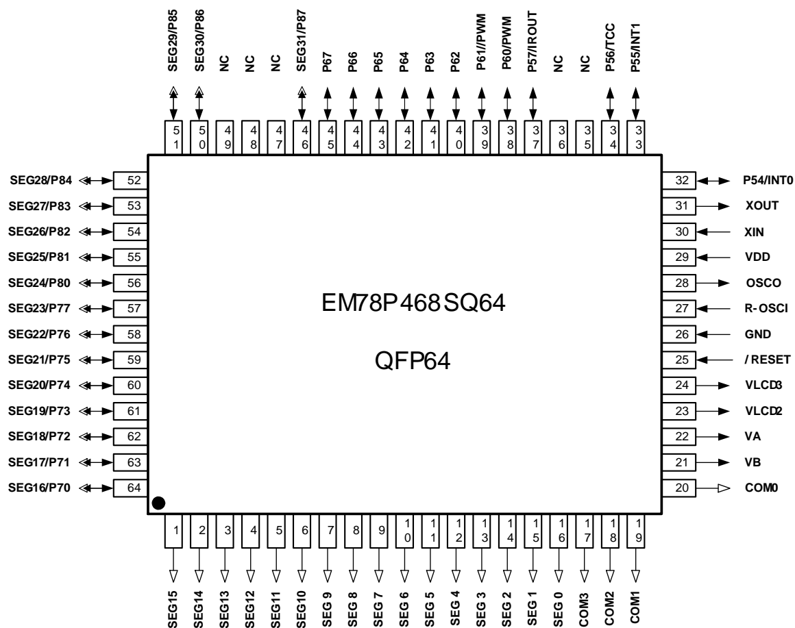
Figure 3-1 64-pin QFP EM78P468SQ64 Pin Assignment
