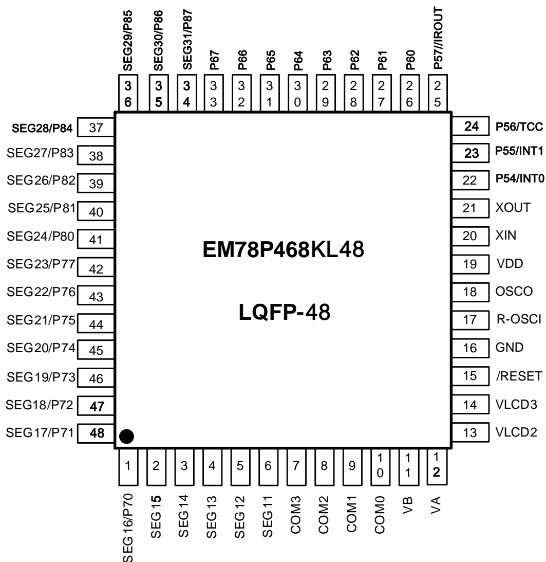
Figure 3-3 48-Pin LQFP/QFP EM78P468KL48 Pin Assignment
