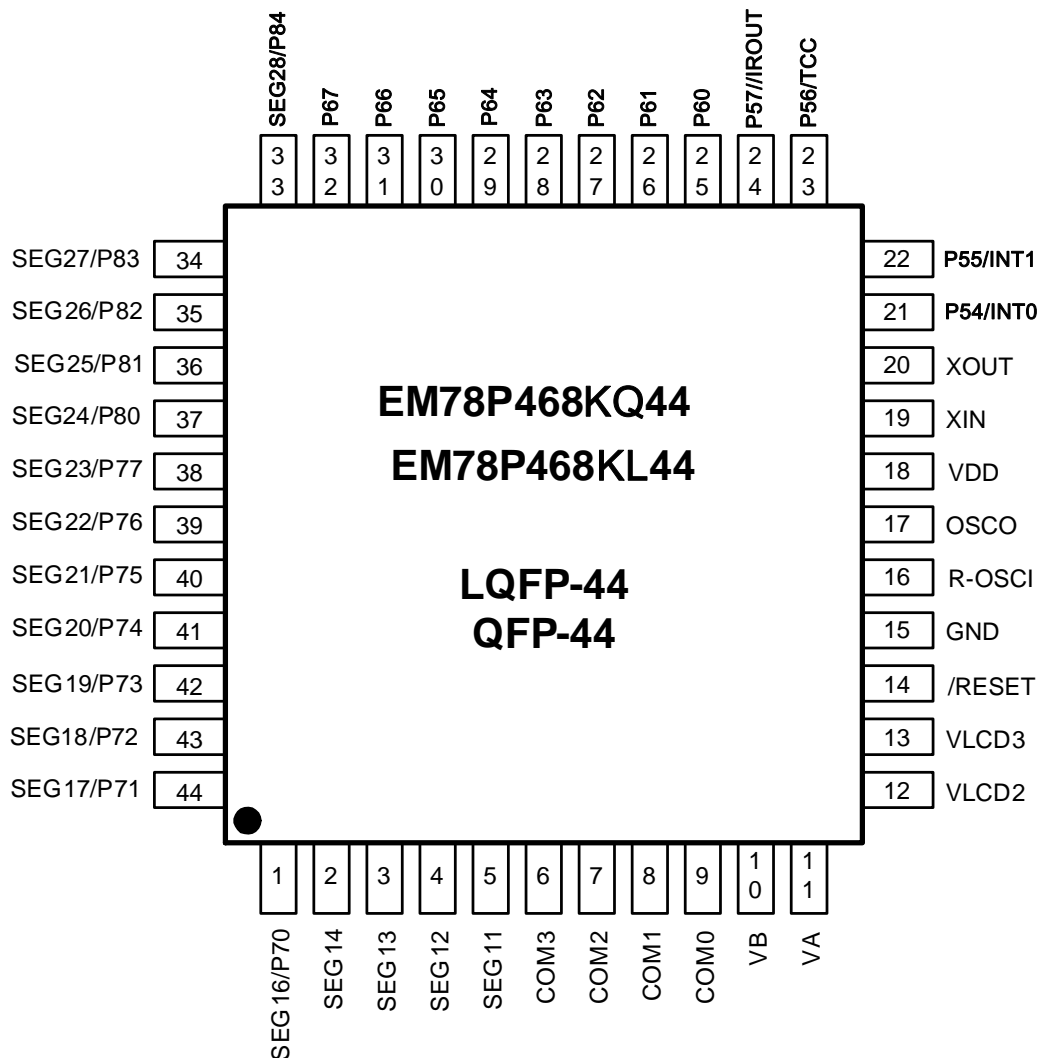
Figure 3-4 44-Pin LQFP/QFP EM78P468KQ44/EM78P468KL44 Pin Assignment
