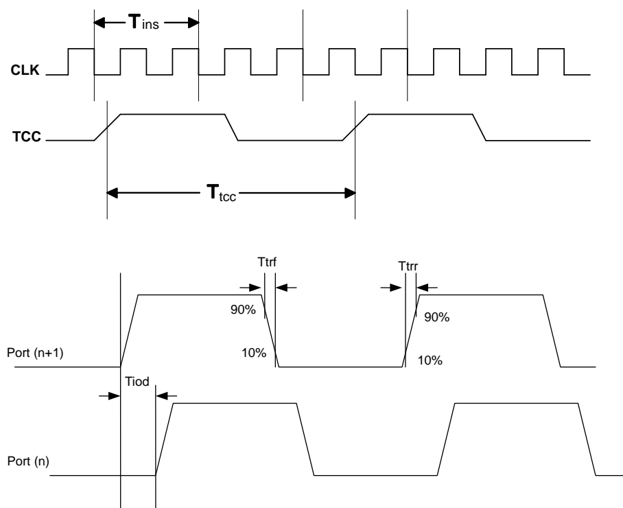
Figure 6-27 Timing Diagrams of EM78P468K
