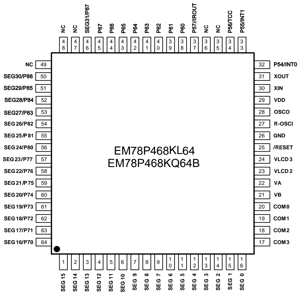
Figure 3-2 64-Pin LQFP/QFP EM78P468KL64/EM78P468KQ64B Pin Assignment
