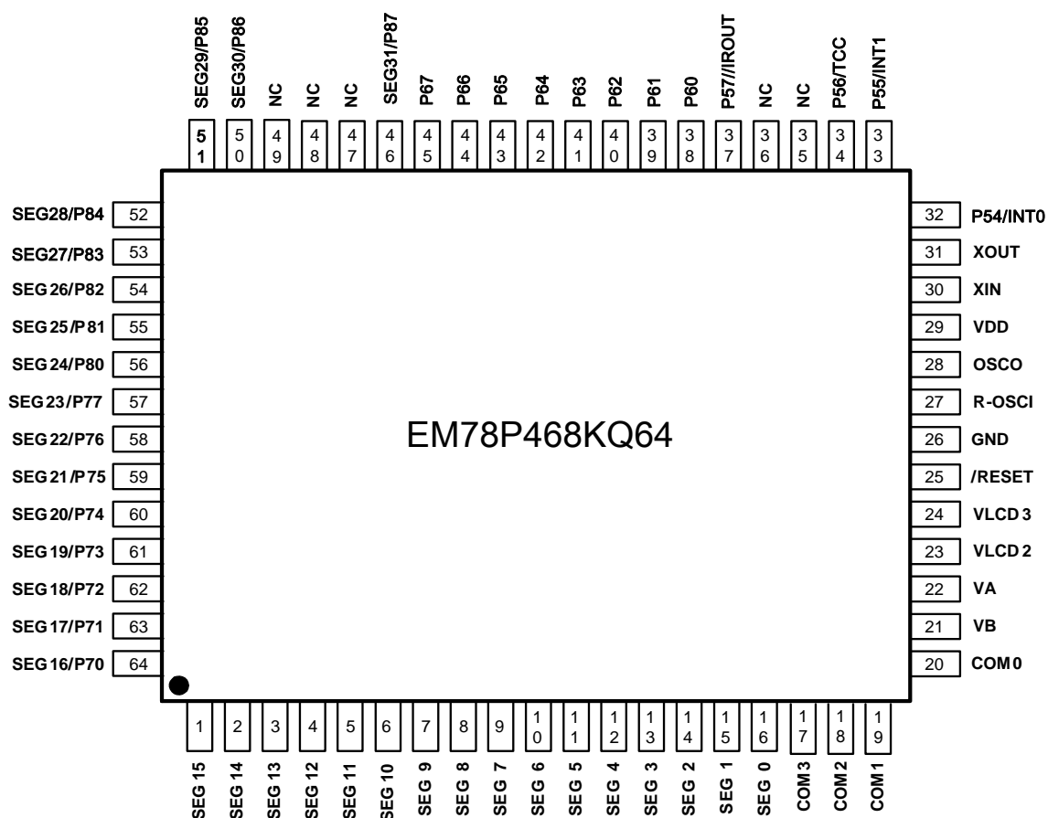
Figure 3-1 64-pin QFP EM78P468KQ64 Pin Assignment
