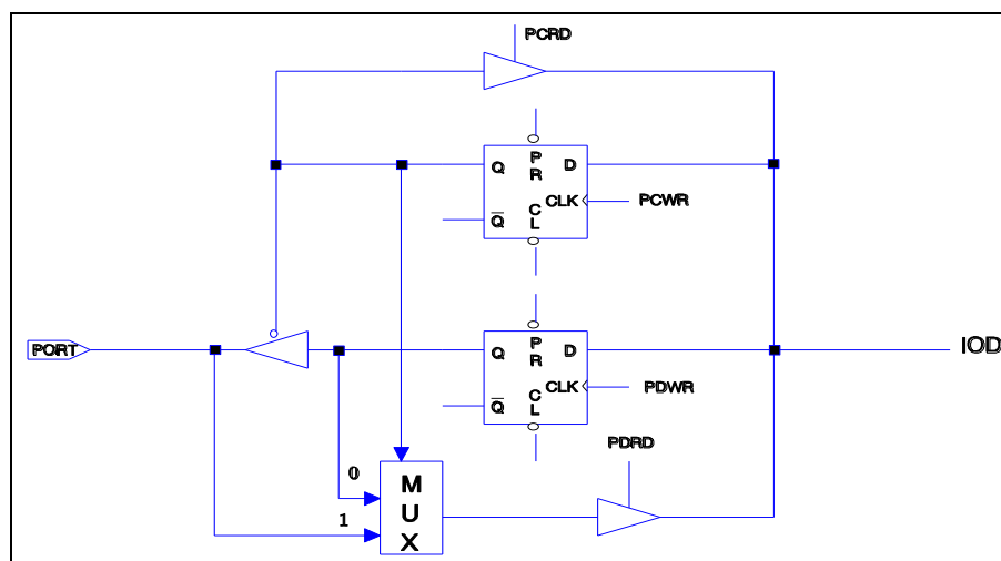
Figure 6-5 Circuit of I/O Port and I/O Control Register for Ports 5 ~ 8
