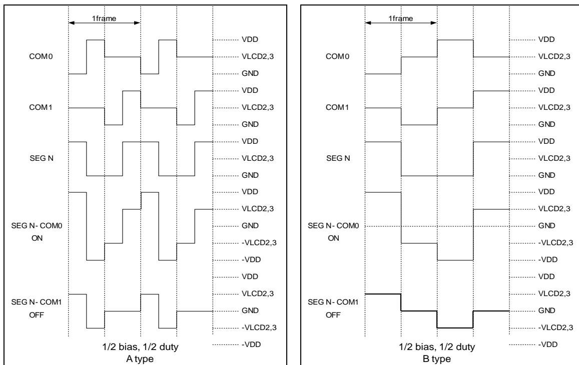
Figure 6-16 LCD Waveform for 1/2 Bias, 1/2 Duty
