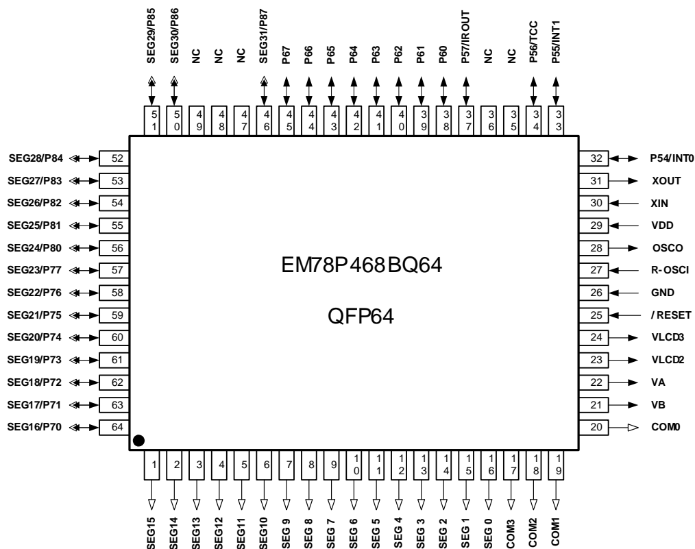
Figure 3-1 64-pin QFP EM78P468BQ64 Pin Assignment
