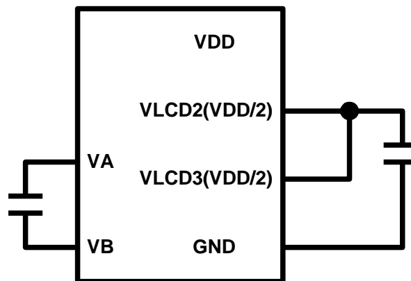
External circuit for 1/2 Bias
