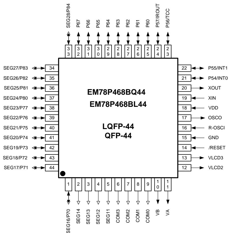
Figure 3-3 44-Pin LQFP/QFP EM78P468BQ44/EM78P468BL44 Pin Assignment
