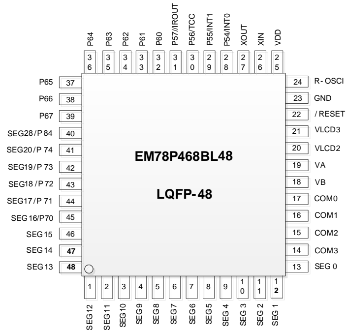
Figure 3-4 48-Pin LQFP EM78P468BL48 Pin Assignment
