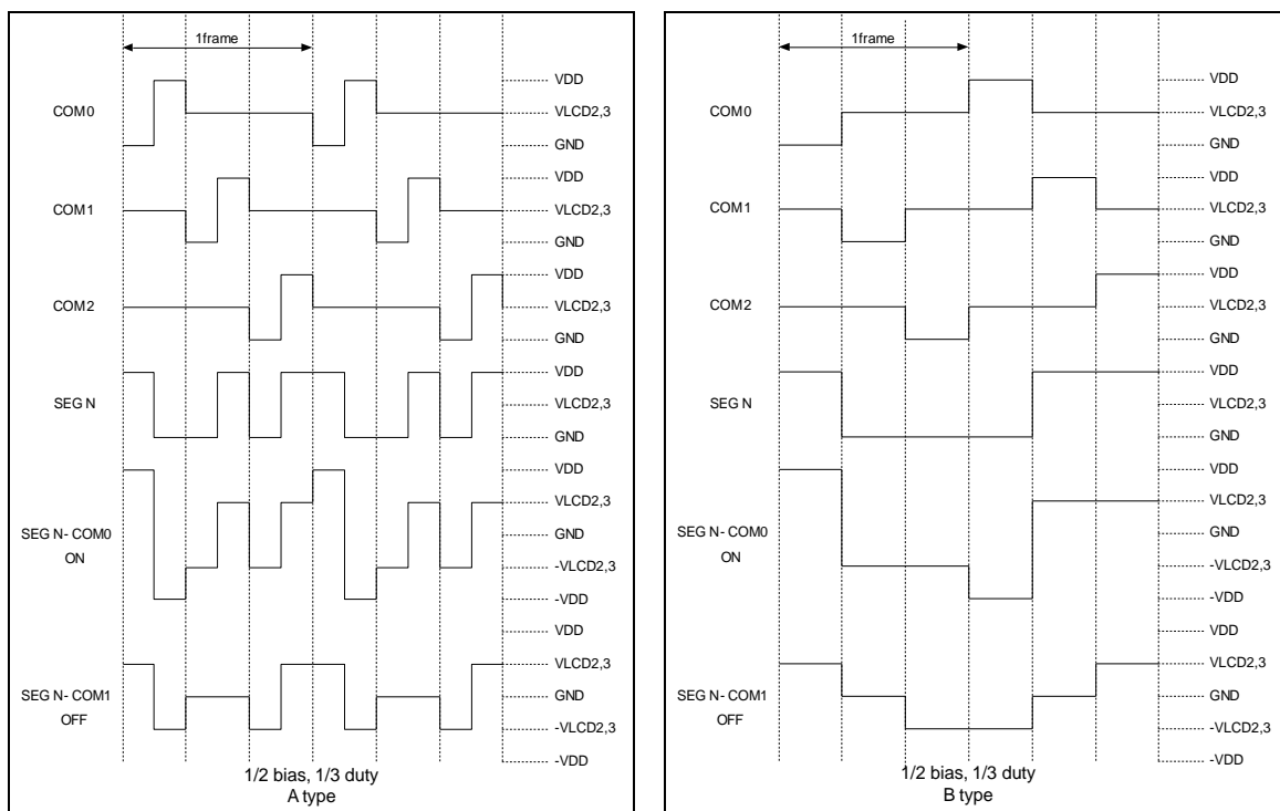
Figure 6-17 LCD Waveform for 1/2 Bias, 1/3 Duty
