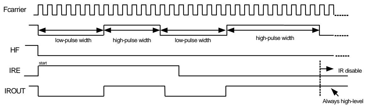
Figure 6-24 LGP=0, IROUT Pin Output Waveform
