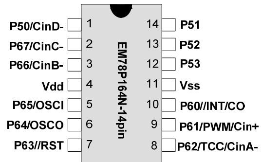
Figure 3-2 EM78P164ND14/SO14
