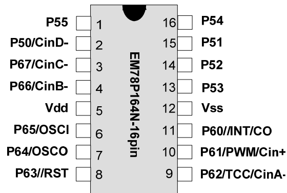
Figure 3-1 EM78P164ND16/SO16
