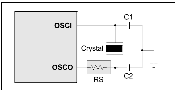
Figure 5-18 Crystal/Resonator Circuit
