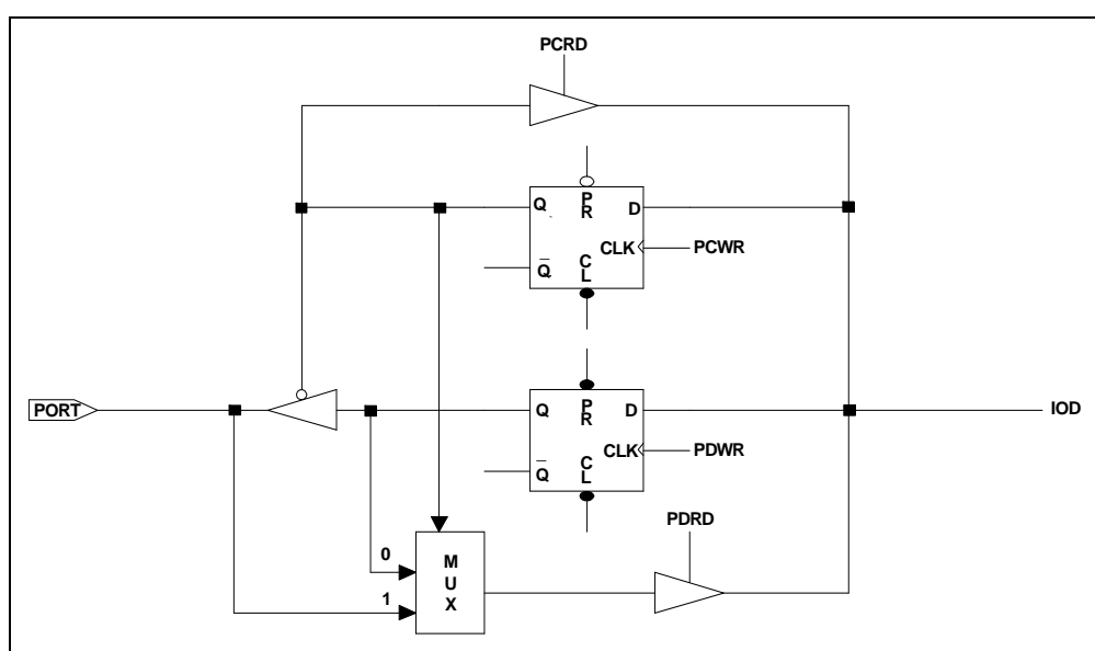
Figure 5-5 The Circuit of I/O Port and I/O Control Register for Port 5
