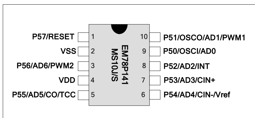
Figure C-3b ICE 143 ICE Cable Connector Pin Assignment
