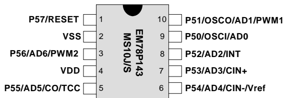
Figure 3-1 EM78P143MS10J/S Pin Assignment
