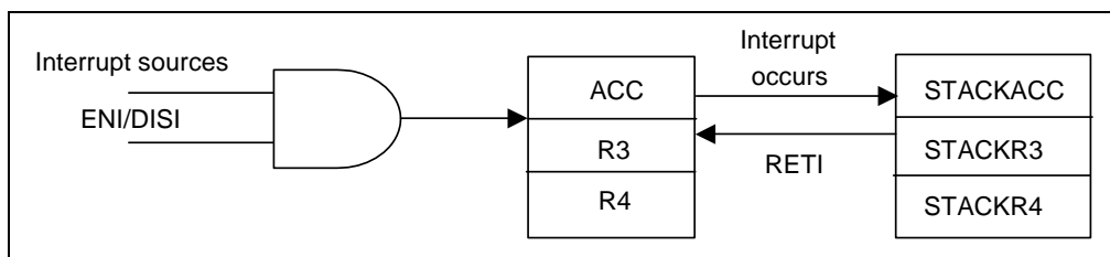
Figure 6-6a Interrupt Backup Diagram
