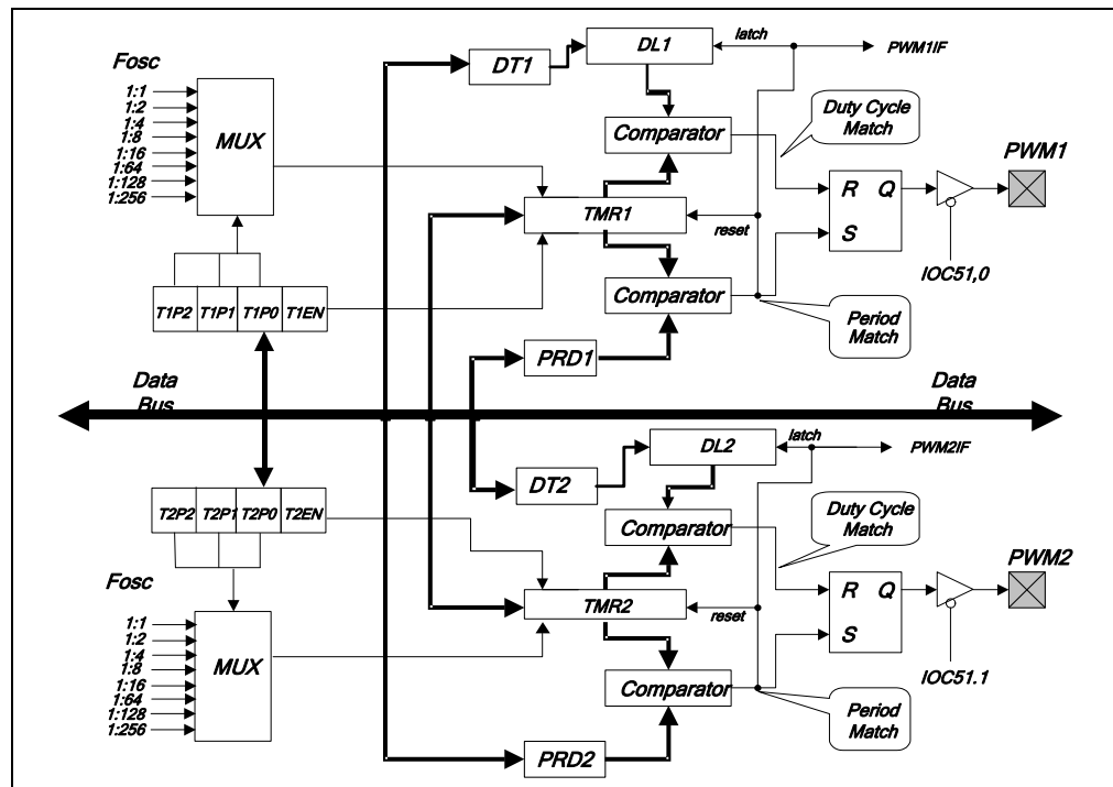
Figure 6-8b Two PWMs Functional Block Diagram
