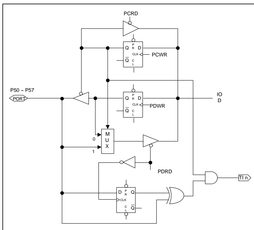
Figure 6-4a I/O Port and I/O Control Register Circuit for Port 5
