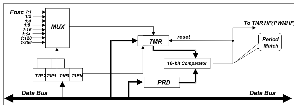
Figure 6-11 16-Bit Timer Functional Block Diagram (Merged from Two 8-Bit Timer)
