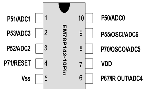
Figure 3-1 EM78P142SS10
