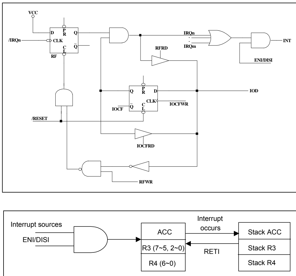
Figure 6-8 Interrupt Back-up Diagram
