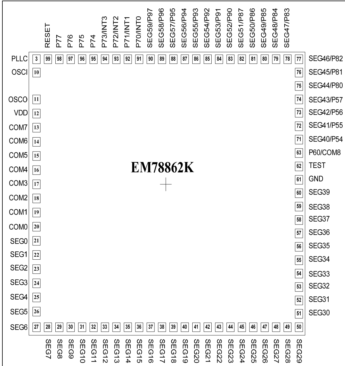
Figure 4-1 EM78862K Pin Configuration for Dice Form
