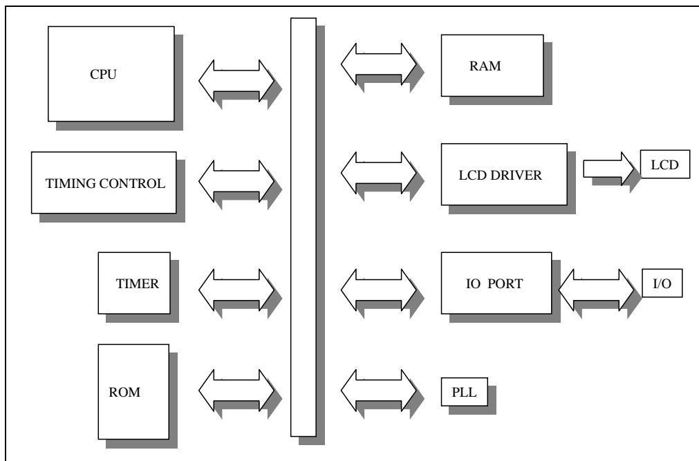
Figure 5-1a System Overview Block Diagram
