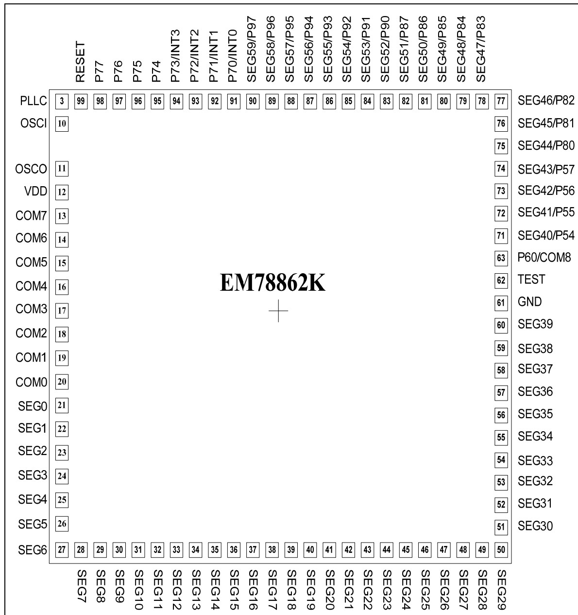
Figure 12-1 WM78862K Pad Diagram and Locations
