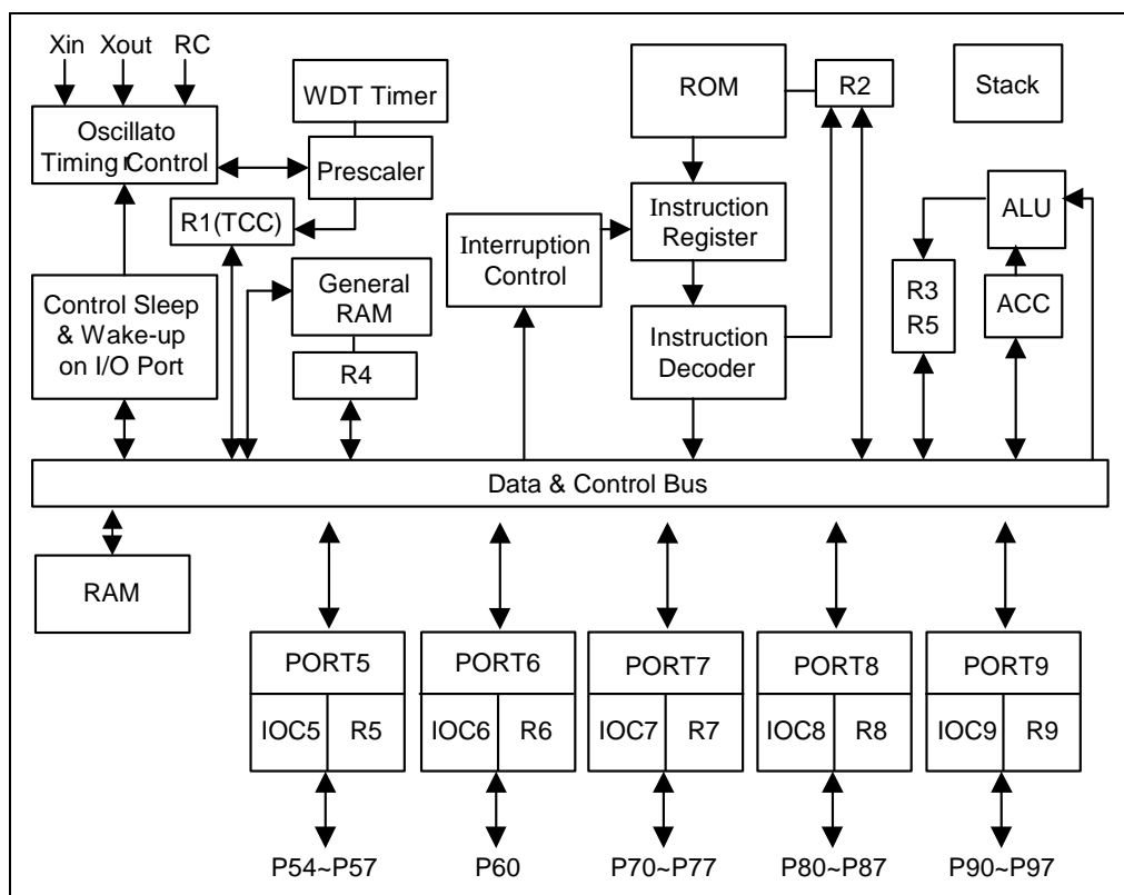
Figure 5-1b System Functional Block Diagram
