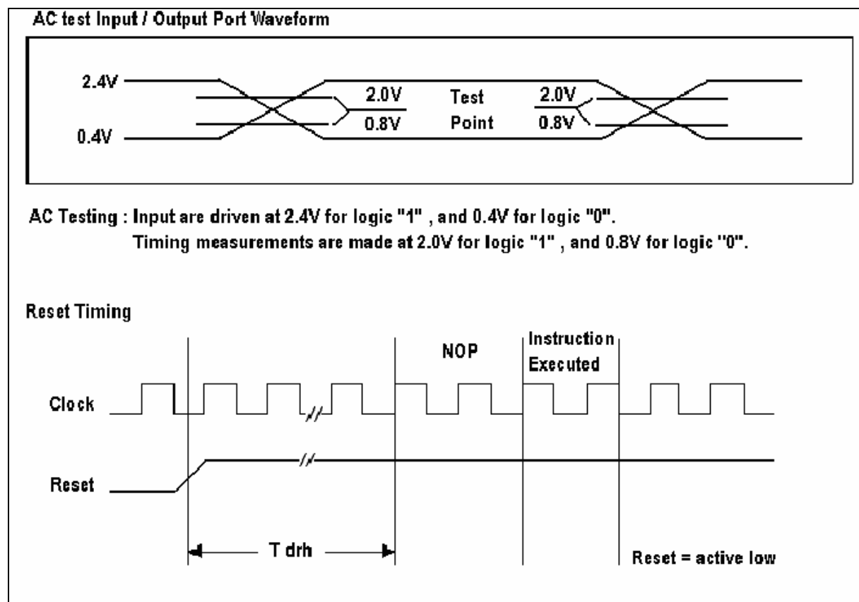
Fig. 10 AC Timing
