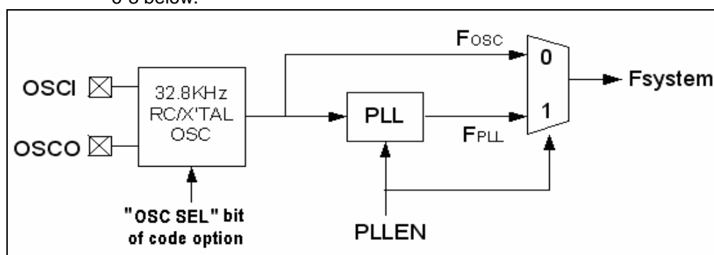
Fig. 6-3 The Relation between 32.768KHz and 3.579MHz
