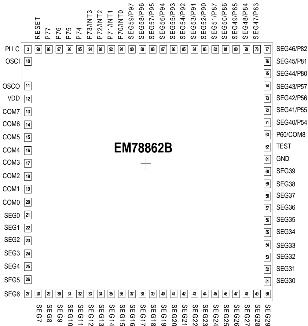
Fig. 4 EM78862B Pin Configuration for Dice Form
