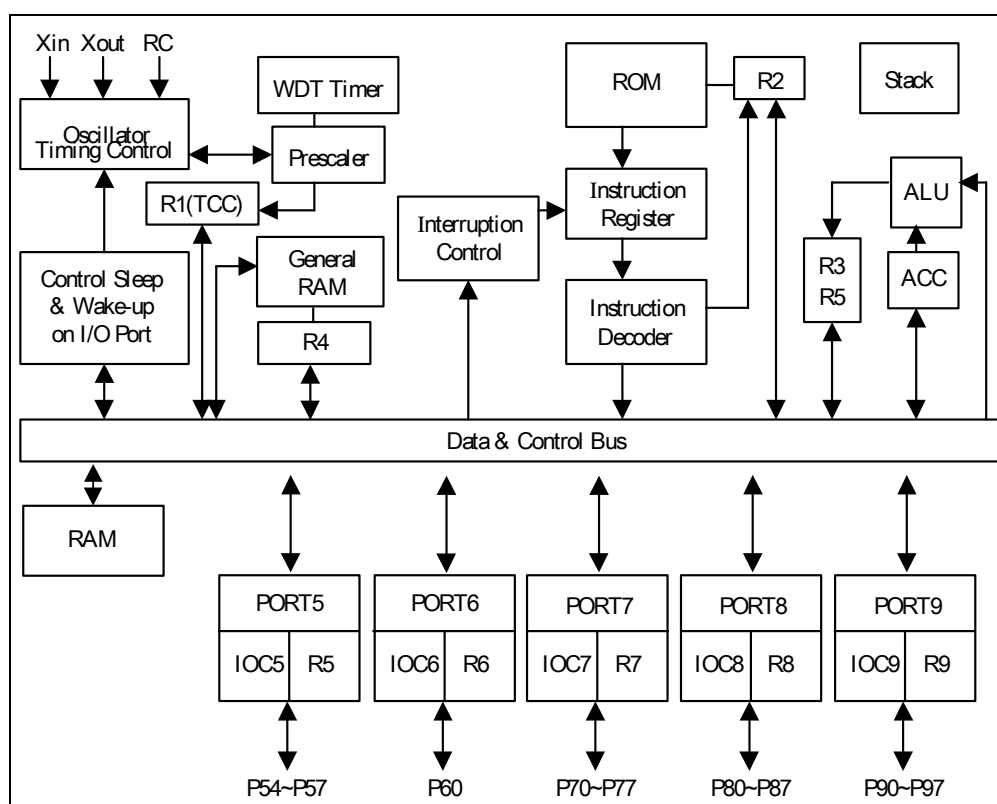
Fig. 5-2 System Functional Block Diagram
