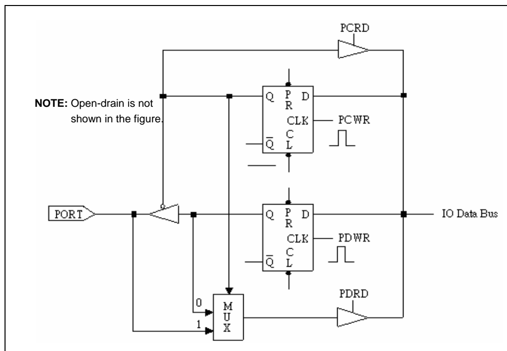
Fig. 6-8 Port 5, Port 6, Port 7, & Port 8 I/O Port and I/O Control Register Circuit
