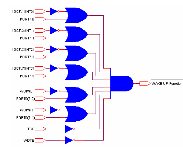
Fig. 6-4 Wake-up Function and Control Signal
