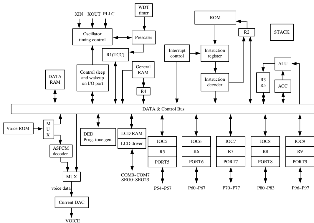
Fig.3 Block diagram2
