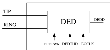
Fig.12 DED diagram
