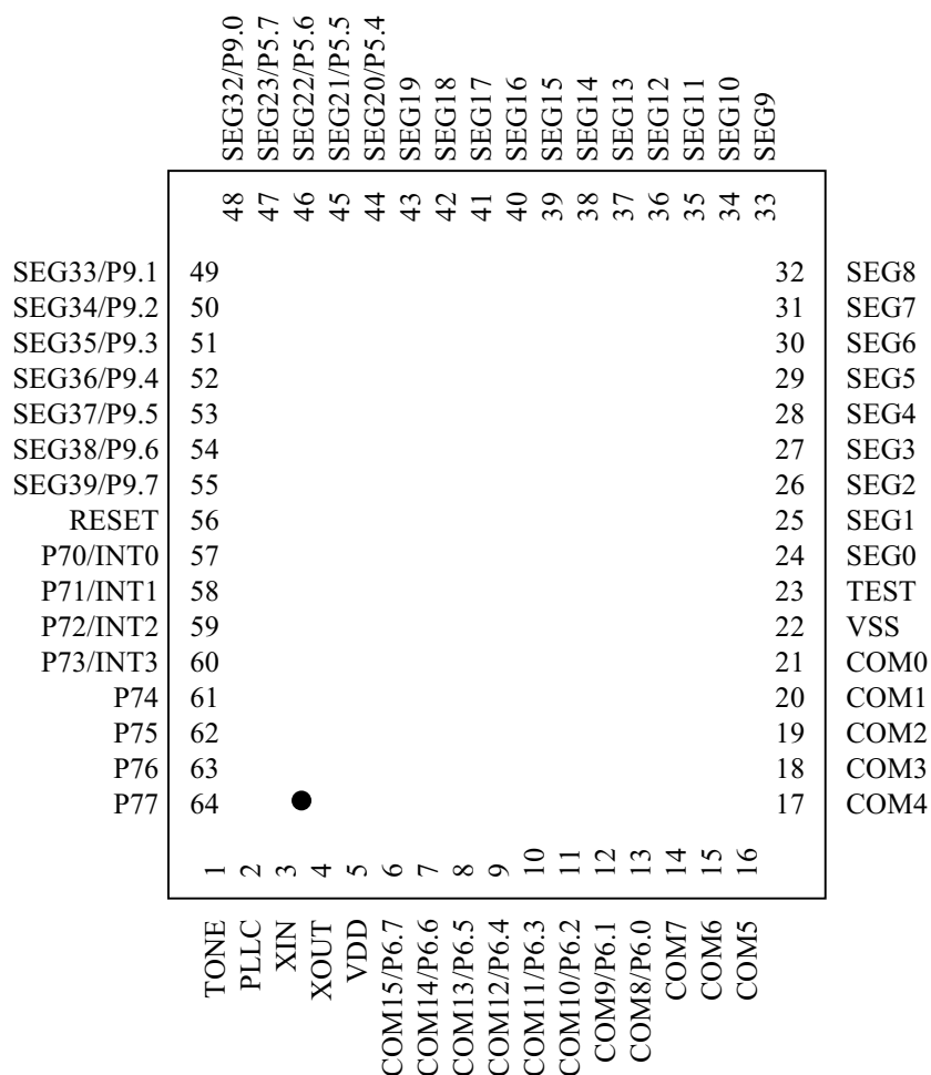
Fig.1 Pin Assignment
