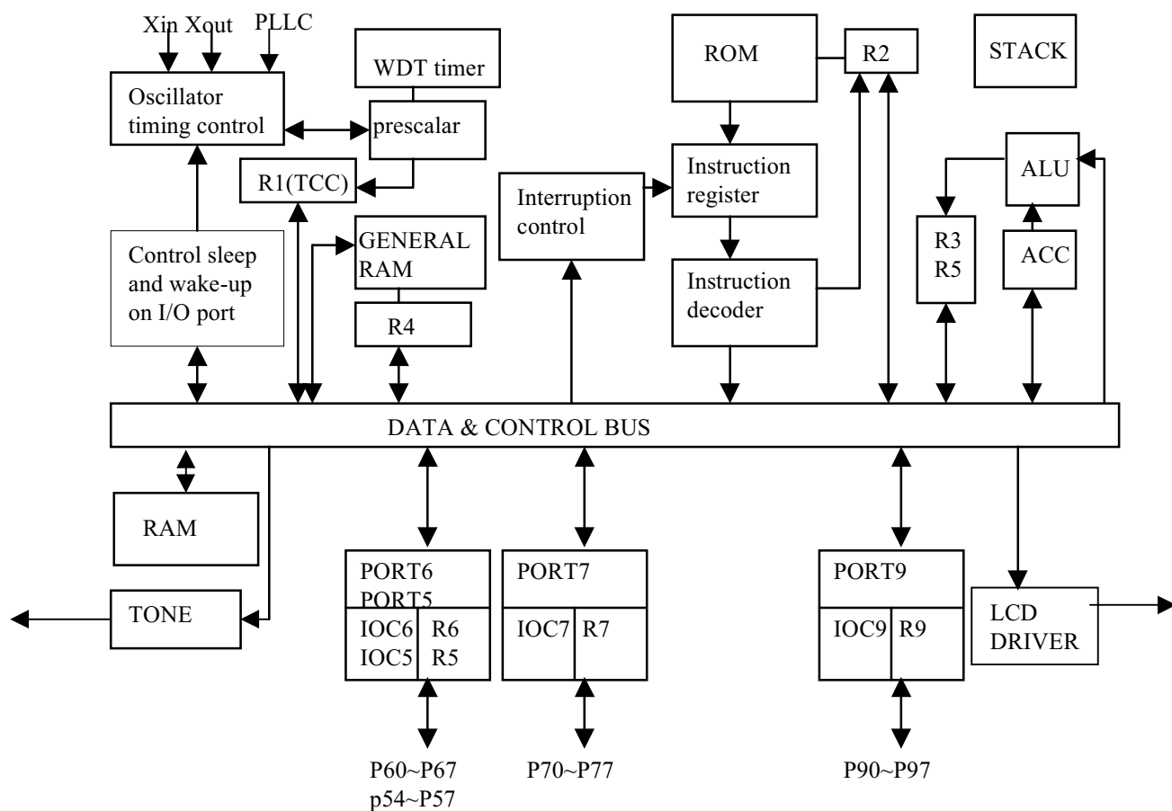
Fig.2 Block diagram
