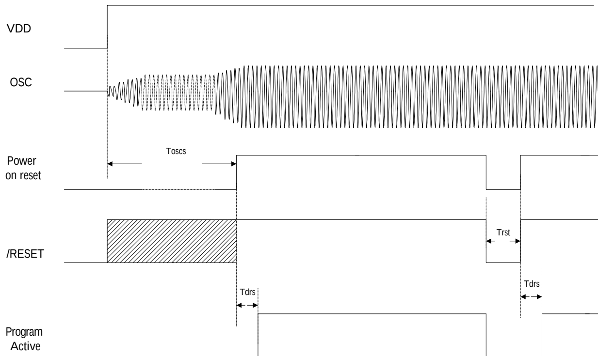
Fig.21 OSC and reset timing
