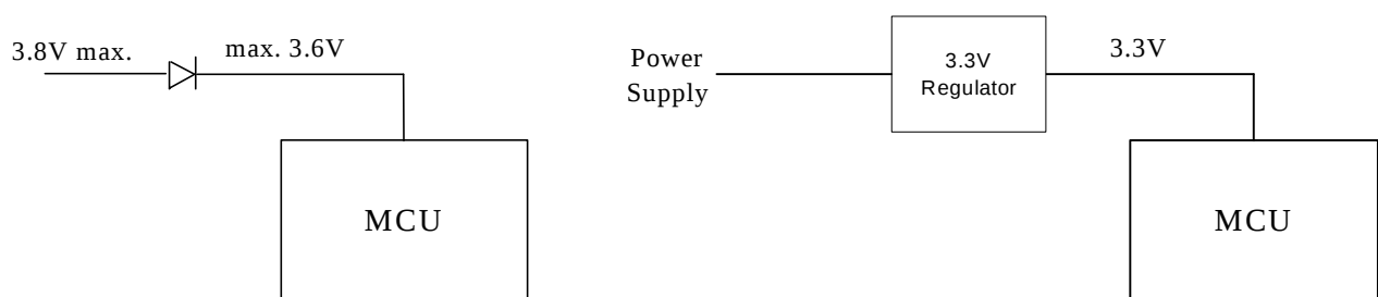
Fig.23 Power Concern in Application
