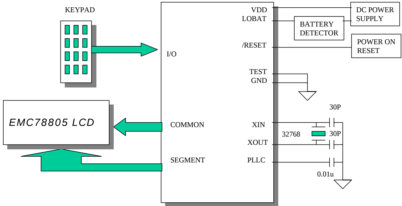
Fig.22 application circuit
