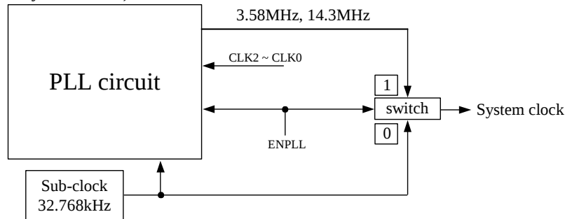
Fig.4 The relation between 32.768kHz and PLL
