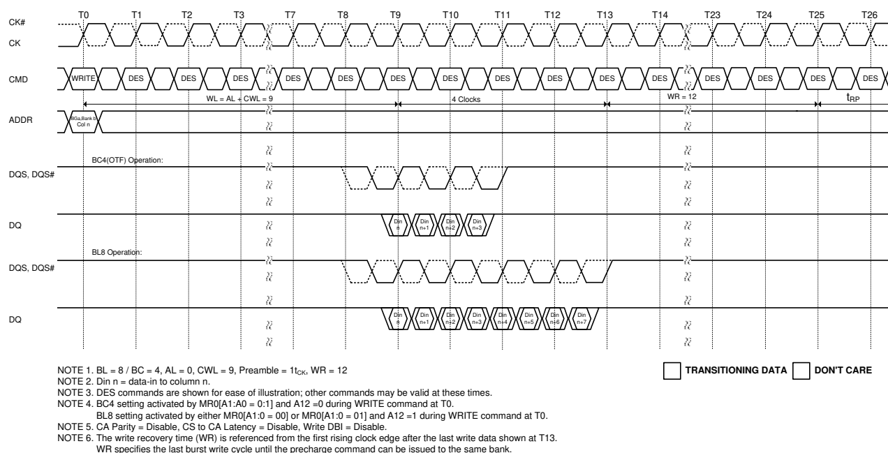
Figure 156. Write (BL8/BC4) OTF with Auto Precharge Operation and 1t_{CK} Preamble
