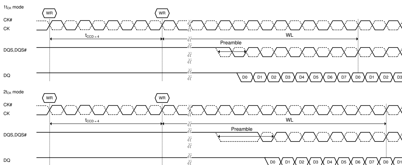
Figure 85. t_{CCD}=4 (AL=PL=0)
