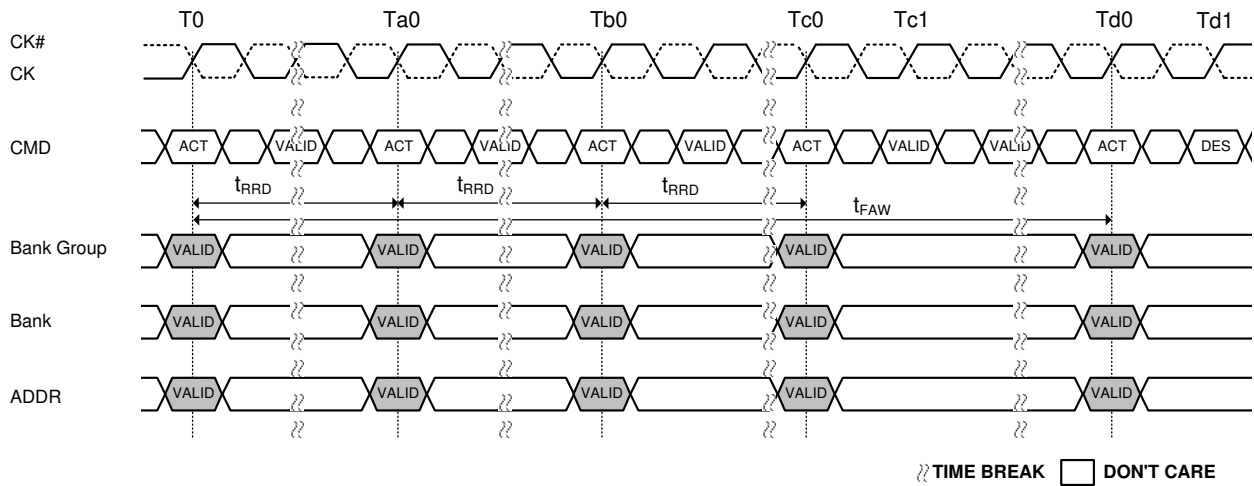
Figure 81. t_FAW Timing
