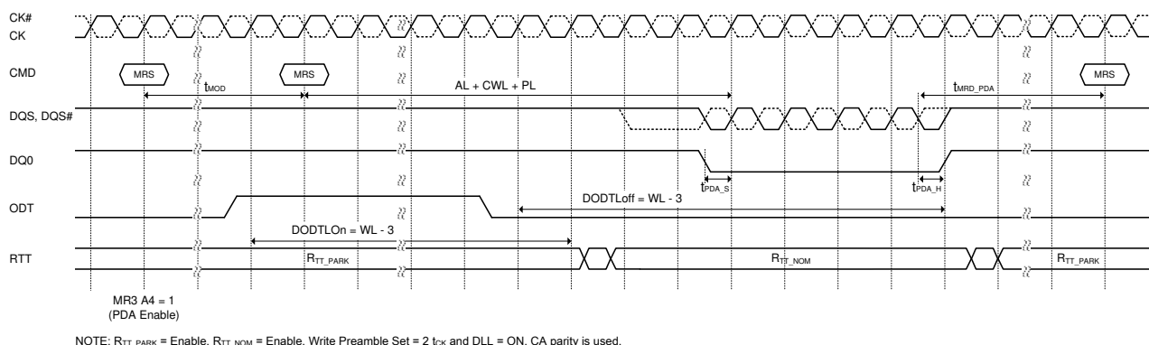
Figure 58. MRS w/ per DRAM addressability (PDA) issuing before MRS
