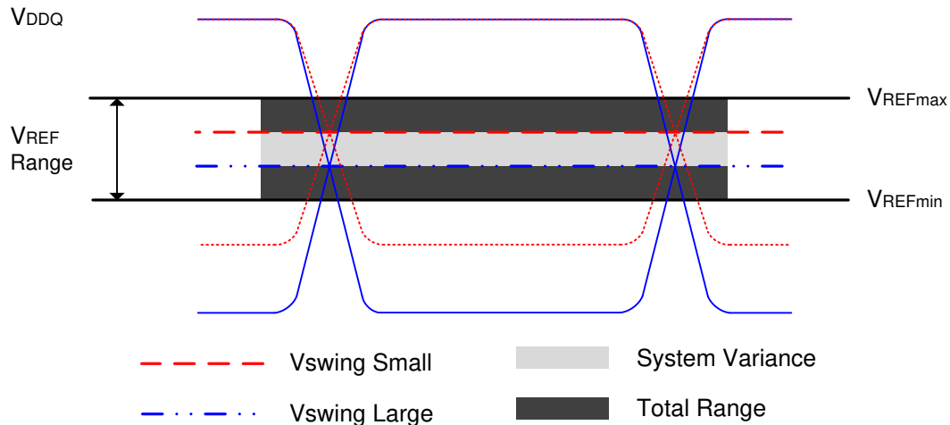
Figure 50. V_{\text{REFDQ}} Operating Range ( V_{\text{REFmin}} , V_{\text{REFmax}} )
