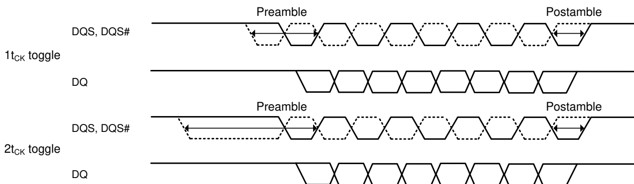
Figure 91. Write Postamble
