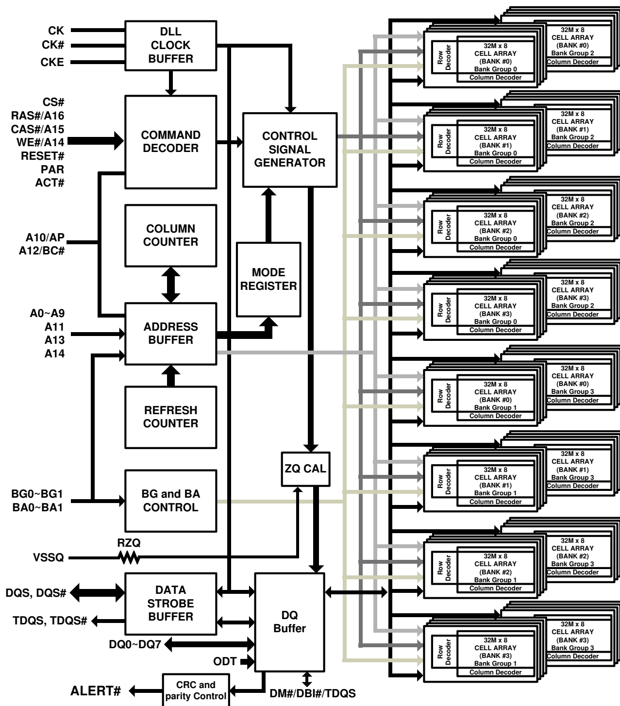
Figure 2. Block Diagram
