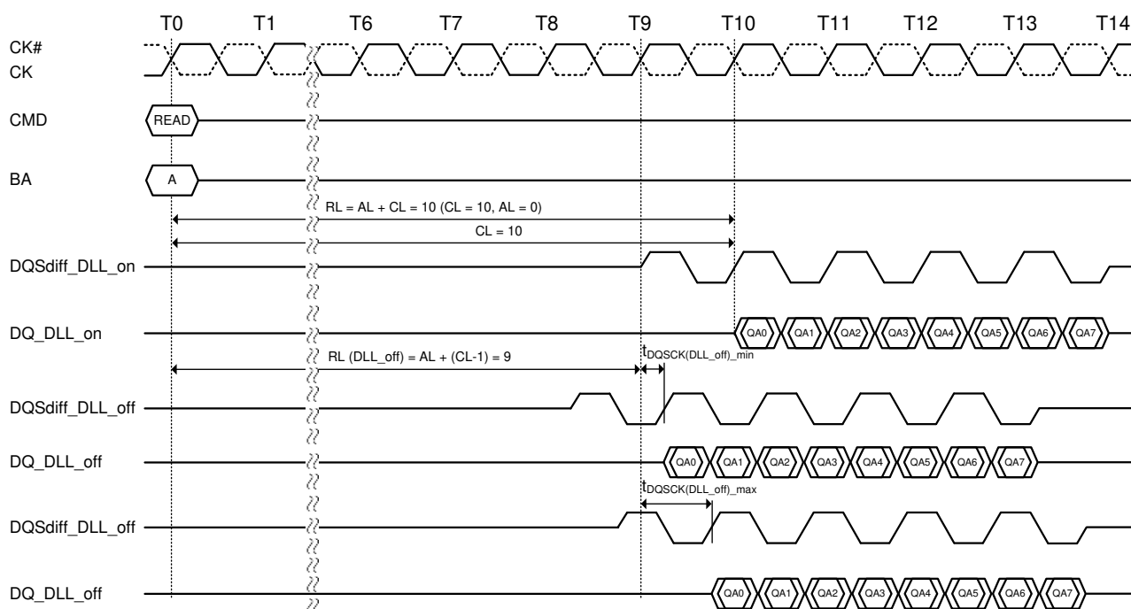
Figure 11. Read operation at DLL-off mode
