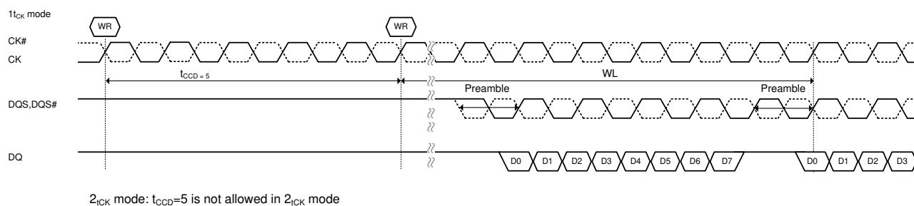
Figure 86. t_{CCD}=5 (AL=PL=0)
