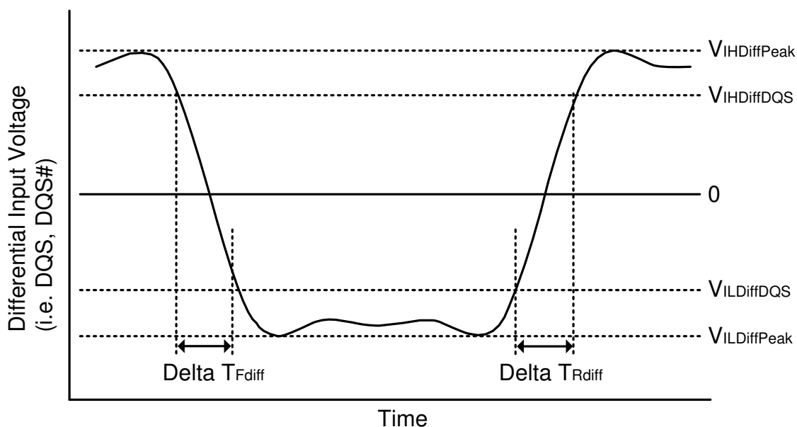
Figure 209. Differential Input Slew Rate Definition for DQS, DQS#
